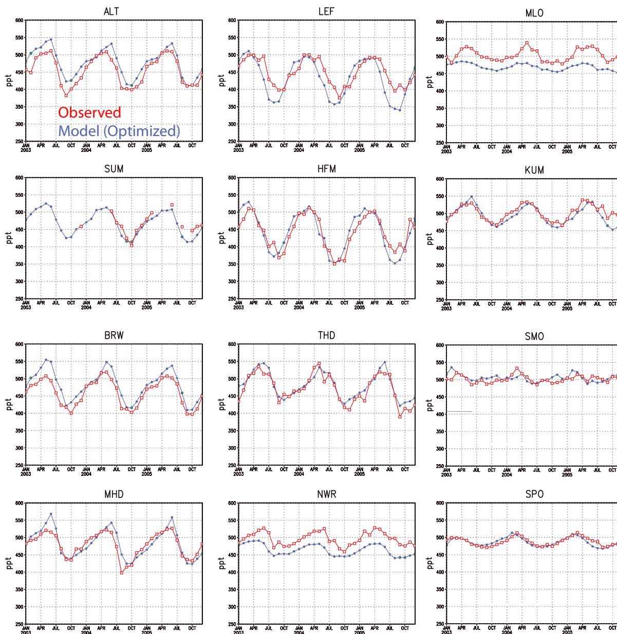
Figure 6. Observations (red) of seasonal variation in COS concentration at the NOAA background atmosphere sampling stations, in comparison with simulations (blue) using revised sources and sinks developed in this paper. Data were obtained from NOAA-ESRL global monitoring network [Montzka et al. , 2007].
