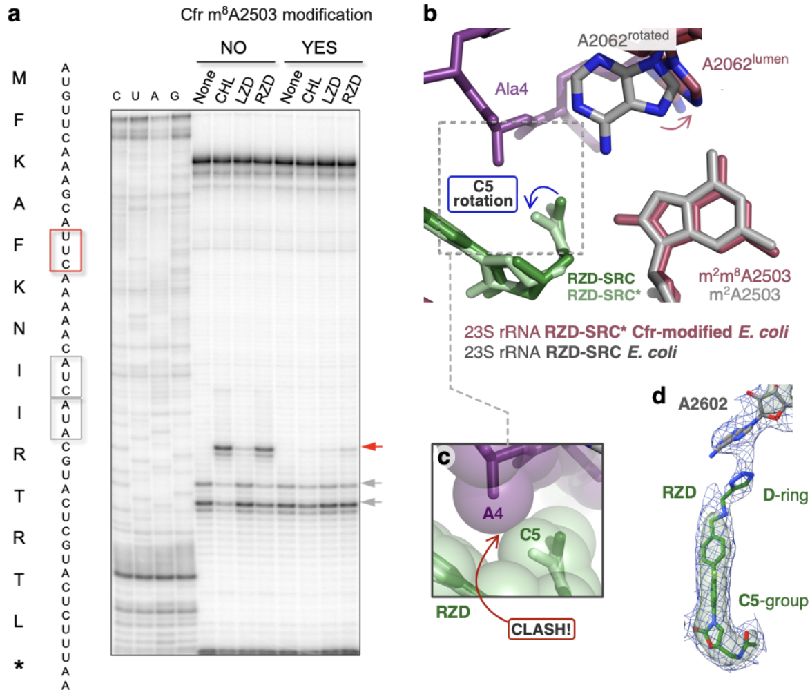
1 2 Figure 4. The Cfr modification m^8A2503 perturbs linezolid and radezolid-induced ribosome 3 stalling. (a) Toeprinting assays performed on the MFKAF stalling peptide sequence. Prominent stall 4 sites observed in reactions containing chloramphenicol (CHL), linezolid (LZD), or radezolid (RZD) 5 with wildtype ribosomes, but not with Cfr-modified ribosomes, are indicated by the red arrow. Due to 6 the inclusion of the tRNA synthetase inhibitor mupirocin in all toeprinting reactions, any ribosomes not 7 stalled at an upstream codon are forced to stall at the Ile codons designated by grey arrows. (b) 8 Structural rearrangements identified in RZD-forced stalled complex with Cfr-modified ribosomes 9 (RZD-SRC*). Stalling peptide in purple is from RZD-SRC. Rotation of the RZD C5 group is required 10 to accommodate m^8A2503 , resulting in a steric clash between the penultimate alanine and the C5 group, 11 close-up view shown in sphere representation in panel (c). (d) Retained interaction between RZD D-ring 12 and A2602 in Cfr-modified ribosomes.
