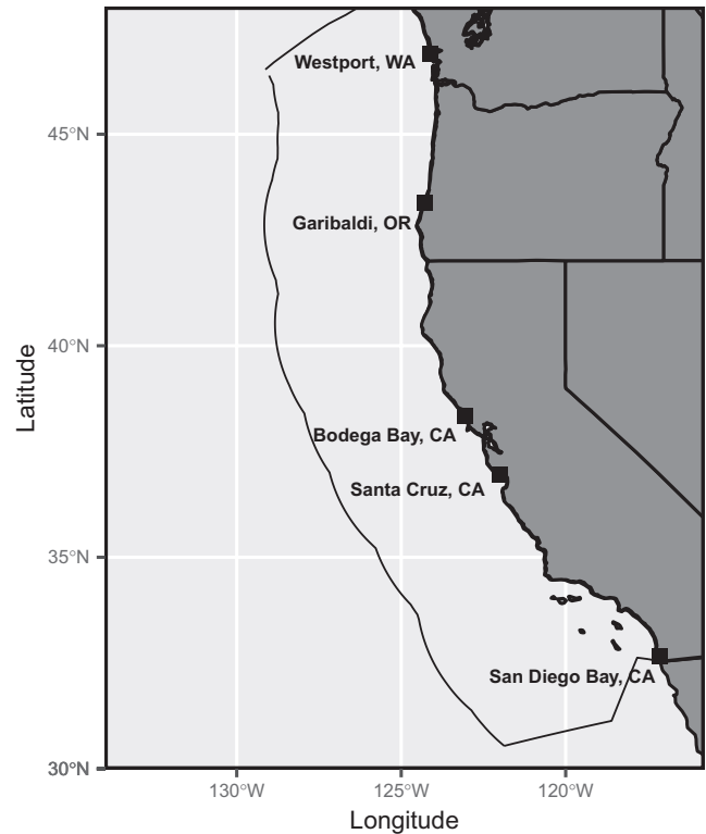
FIGURE 1 Map of the study area, showing the entire ROMS domain. The black outline off the coast of California (CA), Oregon (OR) and Washington (WA) indicates the United States exclusive economic zone (EEZ). The ports used for the distance from port sampling scenarios are labelled and indicated with black squares on the map.
