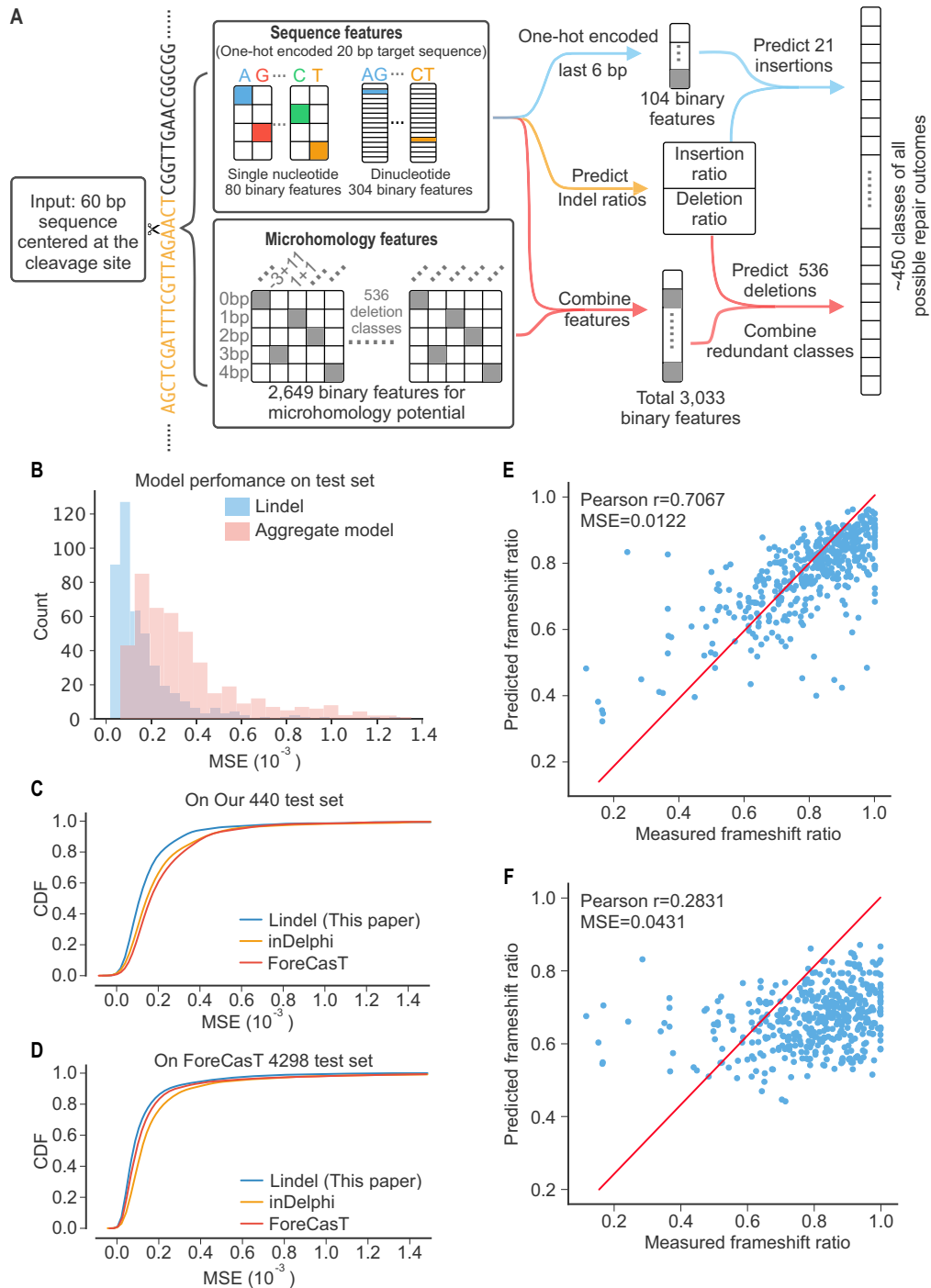
Figure 6. End joining patterns are accurately predicted by Lindel. (A) Schematic of machine learning framework for Lindel. A 60 bp sequence ( \pm 30 bp around the cleavage site) is used as the input to the model. A total of 3033 binary features—2649 corresponding to MH potential and 384 to one-hot encoded mono- and di-nucleotide content of the 20 bp target—are extracted. One-hot encoded sequence features were used to predict overall ratio of insertion to deletion events. One-hot encoded sequence corresponding to the last 6 bp of the target sequence were used to predict 21 insertion classes. Both sequence features and microhomology features were used to predict deletion classes. Probabilities of redundant deletion classes were combined on a sequence specific manner. (B) Performance of Lindel on the test dataset. The distribution of MSE values for the 440 test targets is shown (blue). Poorly predicted targets largely correspond to those that were poorly sampled (see Supplementary Figure S5B). As a baseline to illustrate the improvement conferred by Lindel, we show a similar distribution for the aggregate model, in which the predicted frequencies of 557 indel classes are simply taken from the aggregate frequency at which each is observed in the training and validation datasets (red). (C, D) The performance of Lindel trained using training data aggregated from this study and the ForeCasT study (3900 sequences from this study and 10 725 from (32)). A Lindel model that was trained on the aggregated training datasets performed best on both the test sets from this study (440 sequences) and the ForeCasT study (4298 sequences). (E, F) Lindel (E) compared favorably to Microhomology Predictor (34) (F) in predicting the ratio of frameshifting mutations for each of the 440 targets in the test set.
