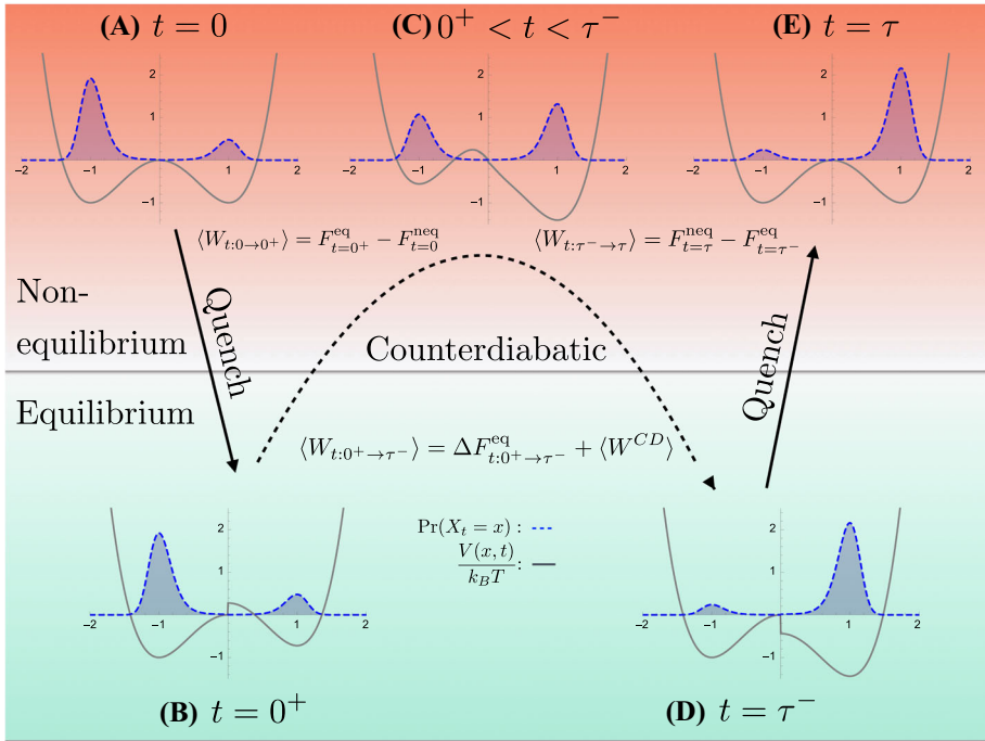
Fig. 3 Counterdiabatic information processing in three steps: Distribution \Pr(X_t = x) shown with blue dashed curves and energy landscapes V(x, t) shown by the gray curves. First, the information landscape is instantaneously changed to fit the starting distribution from stage (A) to stage (B). These share the same distribution but have different energy landscapes. Second, the counterdiabatic protocol is applied to take the system from the equilibrium distribution at stage (B) to that shown in stage (D), passing through nonequilibrium distributions driven from equilibrium by the counterdiabatic potential; such as that shown in stage (C). Third, the last quench step instantaneously takes the system from equilibrium stage (D) to the nonequilibrium metastable stage (E). All three transitions are labeled with the associated work investment
