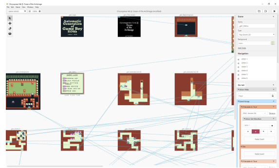
Fig. 2. The GB Studio 1.2.1 interface, displaying the project file for the generated game Crysoypraise Yeti [J]: Ocean of the Archmage . The game is fully editable by the user, and can be compiled into a playable ROM.
