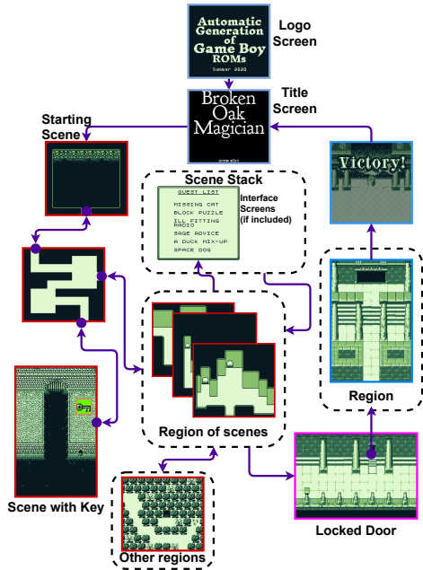
Fig. 3. Diagram of the basic layout of a generated game. Execution begins with the intro and title screens (top left), from which the player can start a new game or load a saved game. New games start in the scene the generator has designated as the starting scene. The scenes are connected via bidirectional trigger links. Connections are tagged with their region, and locked gates are placed between some regions, which can be unlocked by the player finding the matching key. Additional interface scenes (menus, combat, etc.) can be accessed using GB Studio’s scene stack, though the current unified generator doesn’t use that feature.
