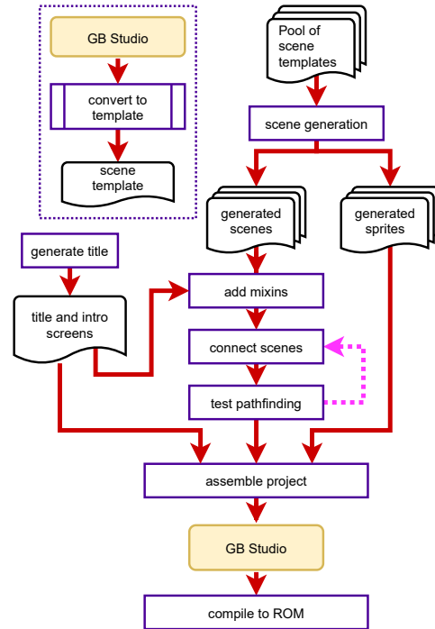
Fig. 4. The generative pipeline in version 1.0 of the generator. The generator starts with a pool of scene templates. The title of the game (generated via Tracery [5]) is used to generate the title screen (via seam-carving [29]), and a MacGuffin is selected based on the title. The MacGuffin and other mixes (such as NPCs) are incorporated into the generated scenes. The scenes are then connected via creating bi-directional links between scenes, with a generate-and-test loop to ensure that the player can pathfind from the start to the end of the game. The generated data is assembled into a project data structure, read into GB Studio, and compiled into a ROM.
