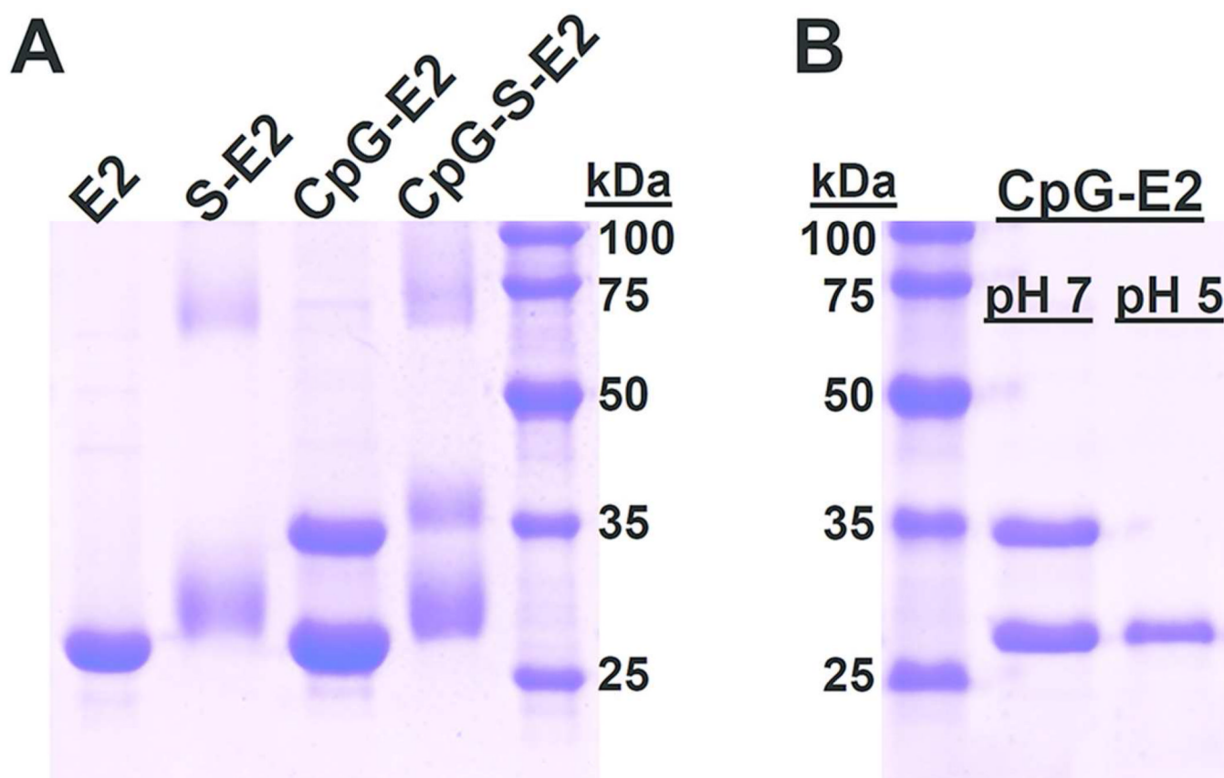
Figure 2. SDS-PAGE of different E2 protein nanoparticles. A) Functionalization of the E2 nanoparticle (E2) with the SIINFEKL peptide (S-E2), CpG 1826 (CpG-E2), and simultaneous conjugation with CpG and SIINFEKL (CpG-S-E2). The unmodified E2 monomer has a theoretical molecular weight of 28105 Da. The 28–32 kDa band in lane S-E2 supports heterogeneous conjugation of the SIINFEKL peptide to the external E2 lysines, with each peptide adding a mass of 1285 Da to the E2 subunit. The CpG-E2 lane displays two bands, corresponding to an unmodified E2 monomer and a CpG-conjugated monomer (34879 Da). The CpG-S-E2 lane shows bands associated with attachment of both CpG and SIINFEKL peptide, supporting simultaneous conjugation. B) Incubation of CpG-E2 at pH 5 results in near-complete hydrolysis of the CpG activator from the E2 monomer. Incubation at pH 7 retains the CpG-E2 conjugate.
