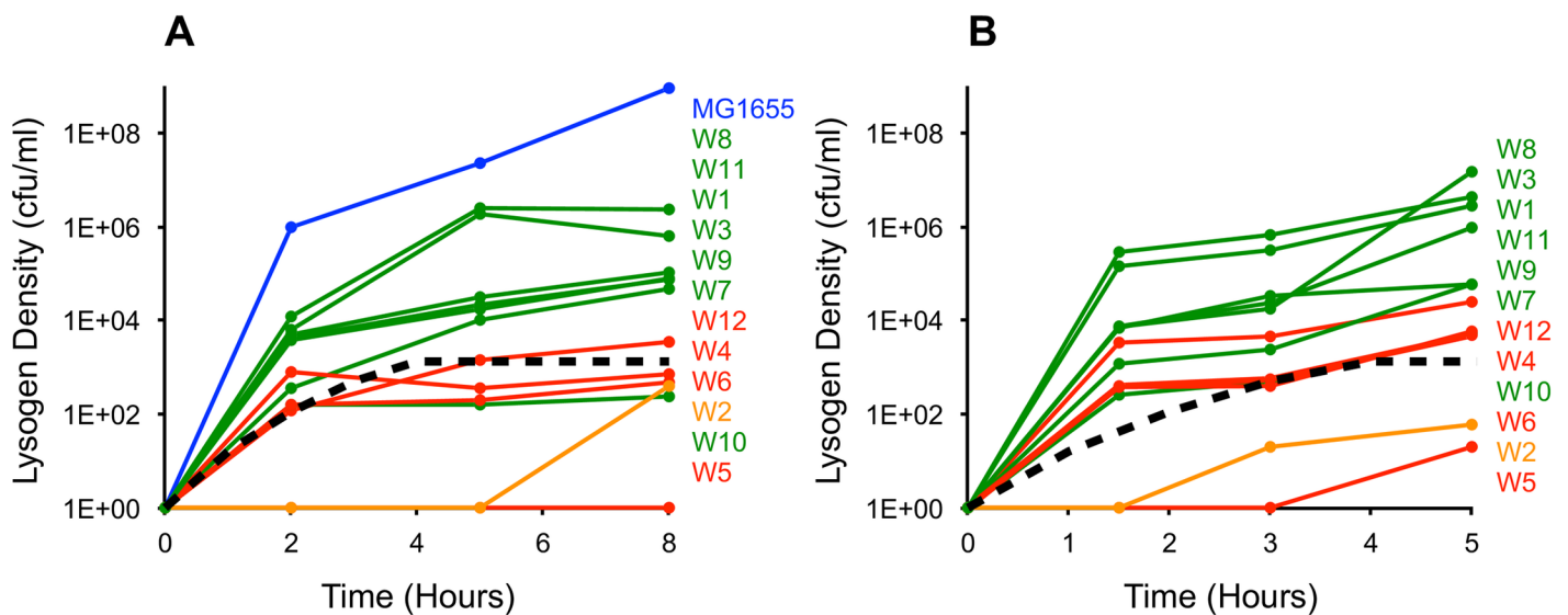
Fig 4. Dynamics of \lambda^{KAN} lysogen formation with 12 independently isolated \lambda^{VIR} -resistant Escherichia coli mutants. (A) and (B) are independent replicates. Green lines correspond to mutants that maintained \lambda^{VIR} in Fig 3A and 3B. Red lines correspond to mutants that did not maintain the phage. W2 is in orange, as it yielded different outcomes. The black dashed lines correspond to numerical solutions of simulations, assuming the rate of transition in the range predicted to be necessary to maintain \lambda^{VIR} ( \mu_N = 10^{-5} ). The remaining parameters were identical to those used in Fig 1, with a probability of lysogeny of \lambda = 0.02 . The labels at the right are ordered according to the final density of lysogens produced. The blue line shows dynamics of lysogen formation in a fully susceptible strain. The experiment with a fully susceptible strain was only performed in one of the two replicates. The final number of \lambda^{KAN} lysogens produced significantly correlated with the ability of \lambda^{VIR} to be maintained on these mutants ( p = 7.9 \times 10^{-4} with 24 observations and 22 degrees of freedom). The p -value was calculated using logistic regression, with the log-transformed number of \lambda^{KAN} lysogens at the end of the experiment as a continuous independent variable and the ability to maintain \lambda^{VIR} (yes/no) as a binary dependent variable. In these statistical tests, it was assumed that W2 cannot maintain \lambda^{VIR} . Assuming that it can maintain the phage still yielded a significant correlation ( p = 0.005 ). Underlying data can be found in S1 Data. cfu, colony-forming unit; \lambda^{KAN} , genetically marked temperate (wild-type) phage \lambda ; \lambda^{VIR} , virulent mutant of phage \lambda .
