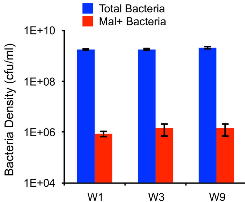
Fig 6. Densities and rate of reversion from Mal - to Mal + in strains W1, W3, and W9. Mean and standard error in total bacterial density ( n = 3 ) and in the number of Mal + mutants ( n = 12 ) are shown. Underlying data can be found in S1 Data. cfu, colony-forming unit; Mal + , phenotype characterized by the ability of bacteria to growth on maltose as a sole carbon source.
