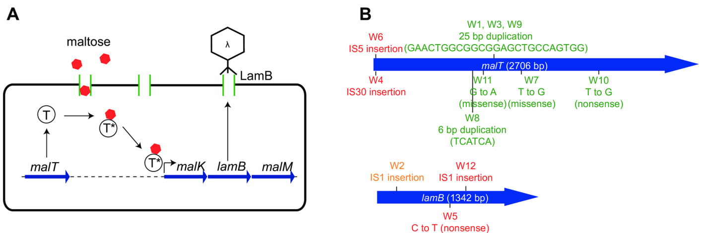
Fig 5. The genetic basis of leaky resistance. (A) Schematics of lamB regulation. Upon binding maltose, MalT serves as a transcriptional activator of the operon containing lamB , which encodes the phage \lambda receptor protein LamB. (B) Mutations identified in the 12 \lambda^{VIR} -resistant strains and their location. Mutations listed in green were found in strains that allowed for stable maintenance of \lambda^{VIR} , whereas those listed in red were found in strains in which \lambda^{VIR} was not maintained. W2, which allowed for phage maintenance in one of two replicate experiments, is shown in orange. \lambda^{VIR} , virulent mutant of phage \lambda .
