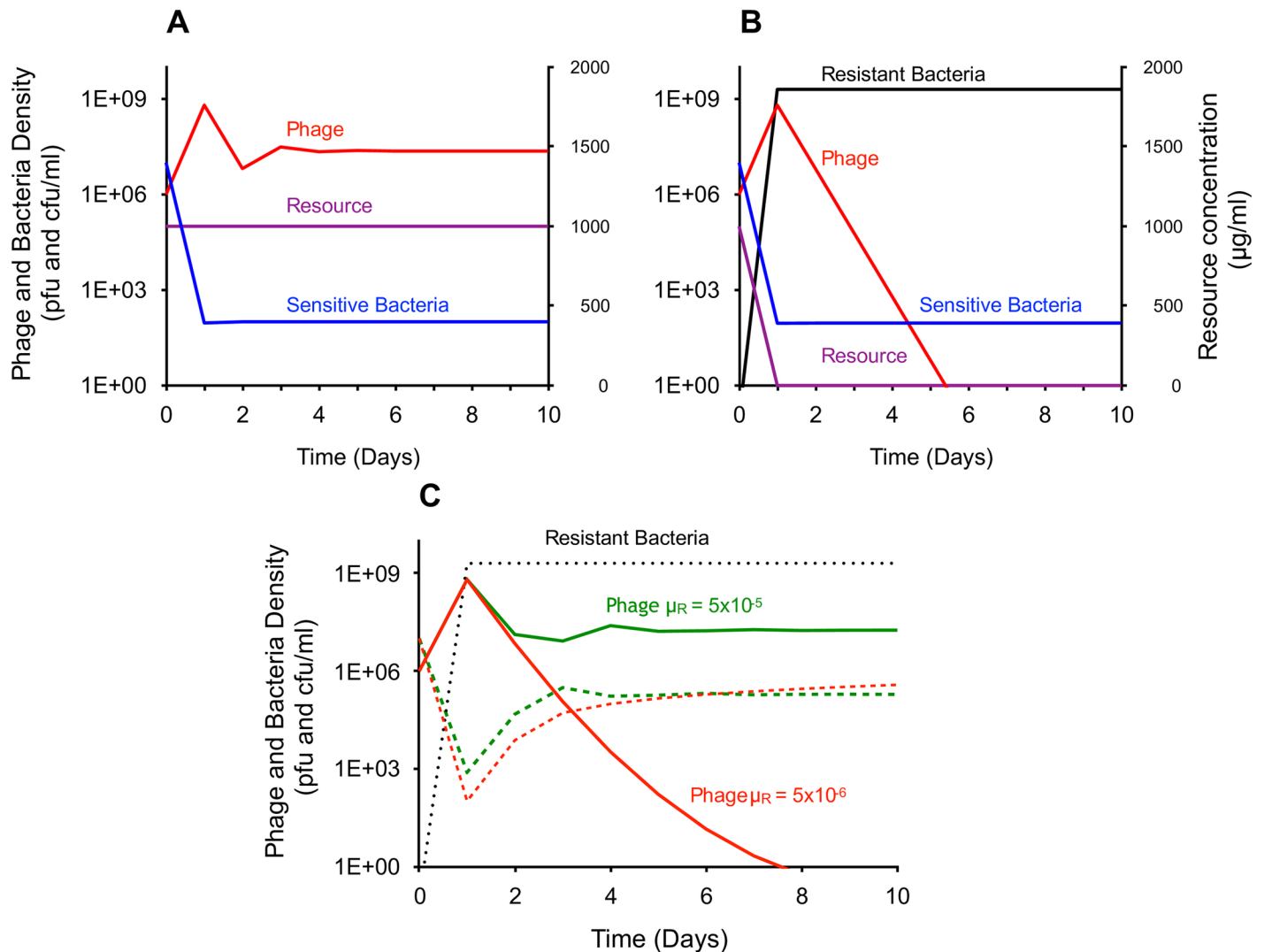
Fig 1. Simulations of population dynamics of bacteria and lytic phage in serial transfer culture. (A) Serial transfer dynamics assuming no transition between susceptible and resistant states ( \mu_N = \mu_R = 0 ) with a refuge of ref = 10^2 . (B) Serial transfer populations considering transition from susceptibility to resistance ( \mu_N = 5 \times 10^{-6} ). \mu_N was estimated independently. Transition from susceptibility to resistance is not allowed ( \mu_R = 0 ). ref = 10^2 . (C) Serial transfer populations considering both transition from susceptibility to resistance and vice versa. Solid curves represent phage densities. Dashed curves represent densities of susceptible bacteria. The black dotted line represents density of resistant bacteria for both simulations. Resource concentration is not shown. In all simulations, densities are plotted at the end of each transfer. Parameters used: v = v_r = 1 , k = 1 , \delta = 2 \times 10^7 , \beta = 60 , C = 1,000 , e = 5 \times 10^7 . The parameters were estimated independently in LB medium. The simulations were initiated with 10^7 susceptible bacteria and 10^6 phage. The models were solved numerically using the Berkeley Madonna software. Copies of this and the other program used in this study are available at www.ecdf.net . Underlying data can be found in S1 Data . cfu, colony-forming unit; LB, Lysogeny broth; pfu, plaque-forming unit.
