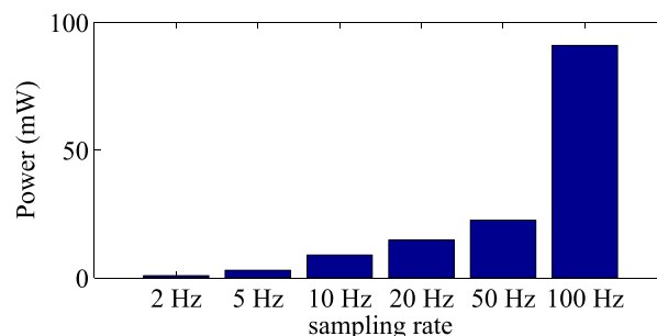
FIGURE 9. Power consumption of smartphone (with display, network and other apps off) reading individual accelerometer sensor signal at different sampling rates.
