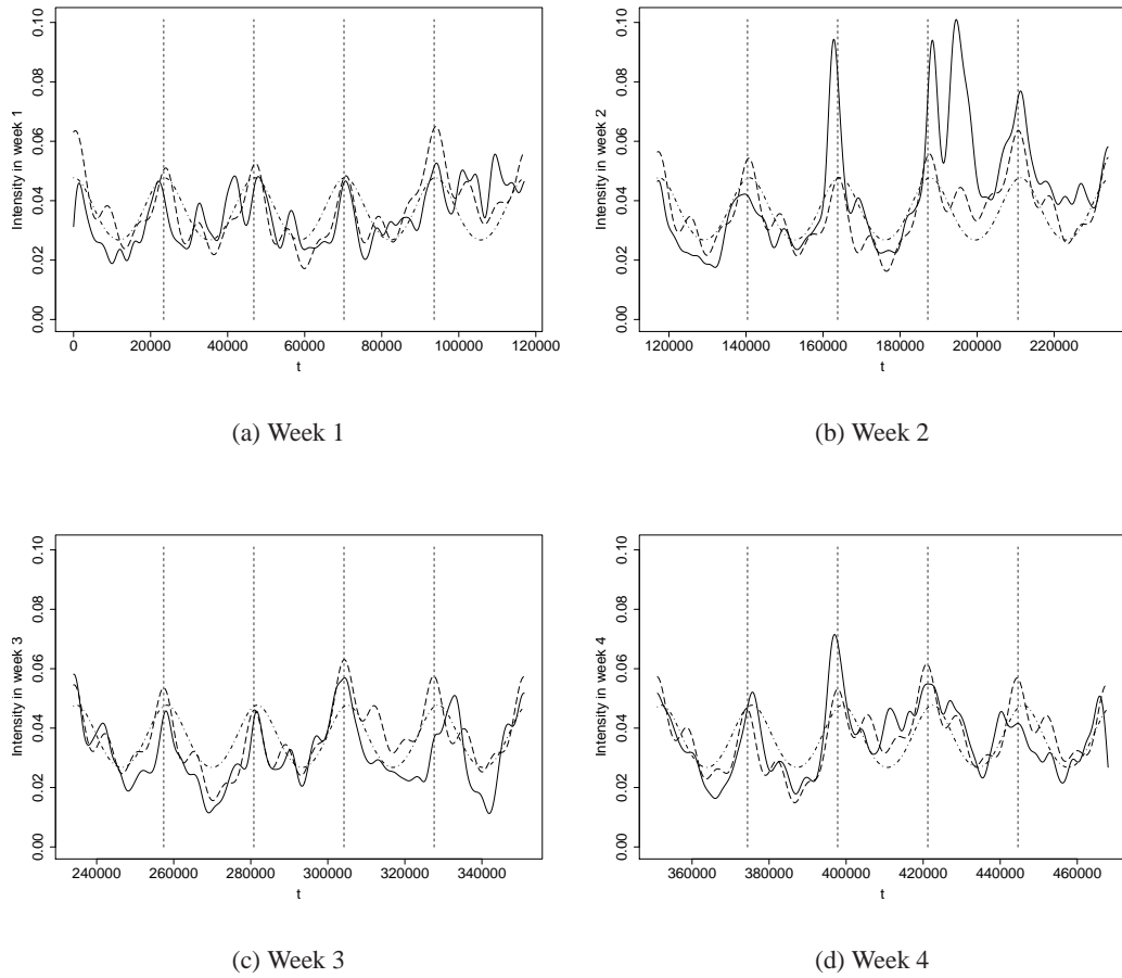
Figure 2.6: Solid line: the non-parametric estimate of the intensity function. Long dashed line (---): the estimated intensity function using our model (2.3). Dotdashed lines (· - · -): the estimated intensity function using model (2.1). The vertical light dashed lines separate days in each week.
