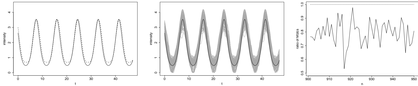
(a) Solid line: true intensity function. Dashed line: estimated intensity function from one replicate.
