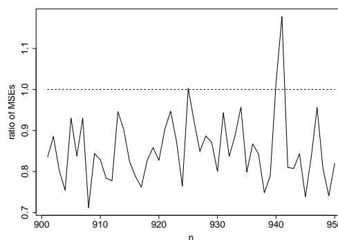
(b) AP vs HPP
