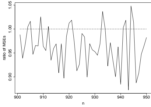
(a) AP vs Vere-Jones(1982)
