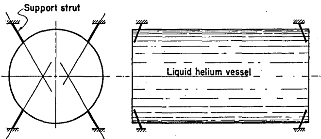
Figure 7. Quadrupole helium-vessel support system; schematic
