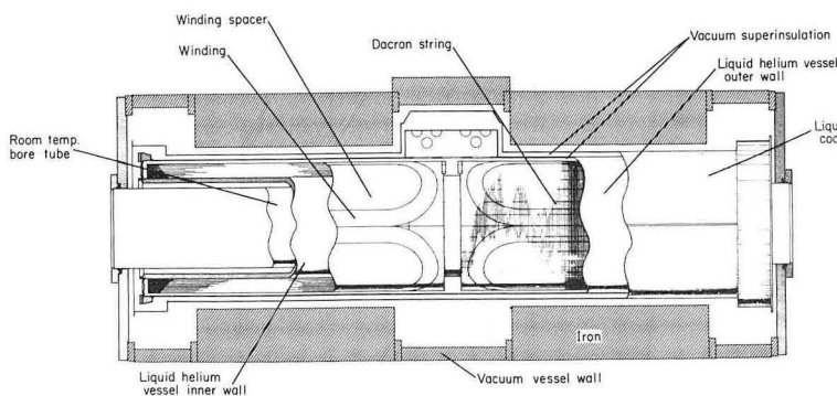
Figure 2 Superconducting quadrupole doublet
