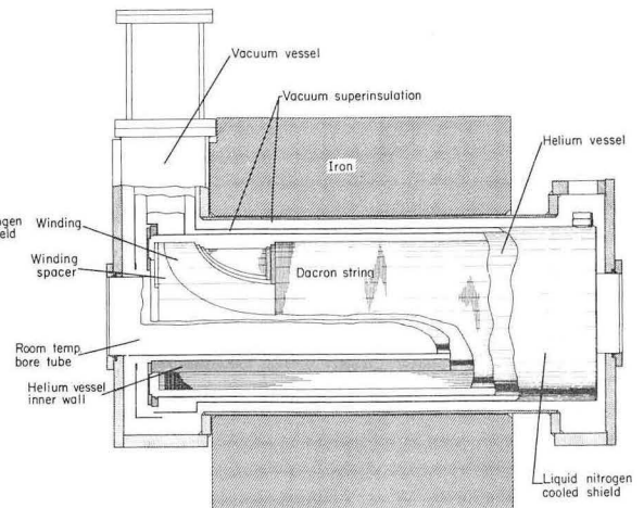
Figure 1 Superconducting dipole magnet
