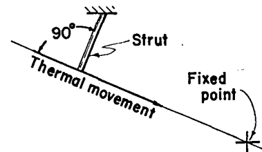
Figure 9 Strut arrangement for zero thermal stress
