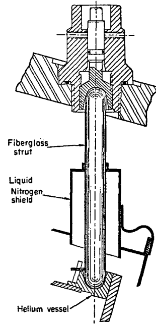
Figure 8 Quadrupole support-strut detail
