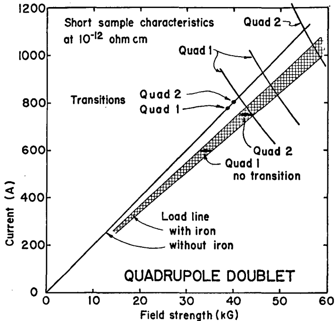
Figure 5 Load lines and short-sample characteristics; quadrupole doublet
