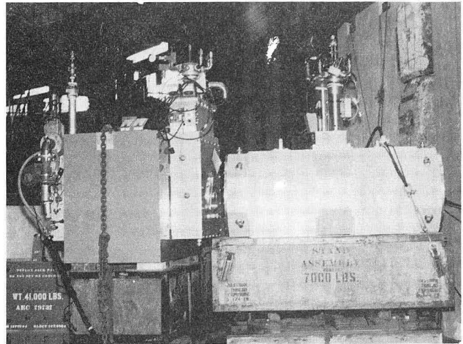
Figure 3 The magnets during installation at the Bevatron
