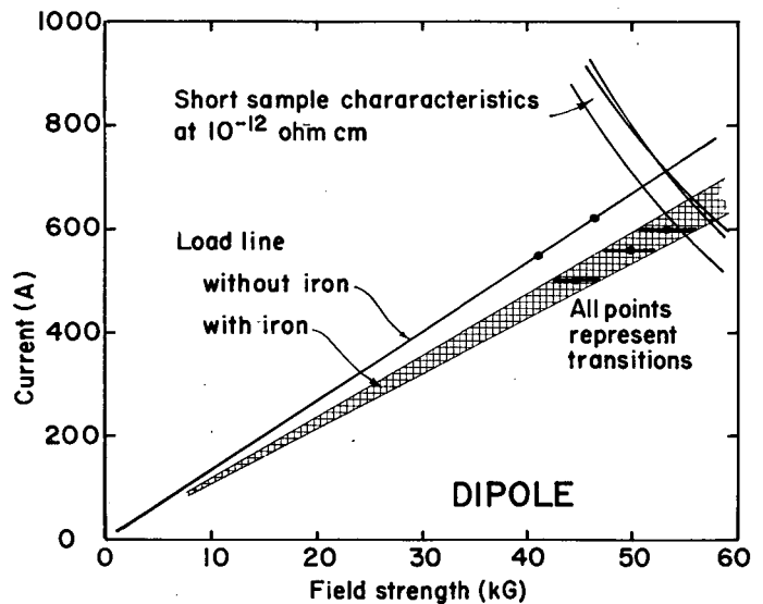
Figure 4 Load lines and short-sample characteristics; dipole.
