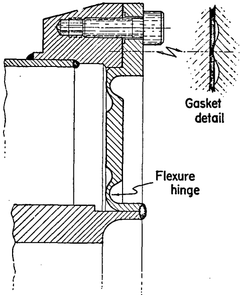
Figure 6 Quadrupole helium-vessel closure
