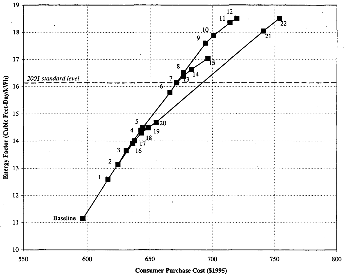
Figure 5.3. Cost Versus Efficiency for New Top-Mount, Auto Defrost Refrigerator-Freezer
