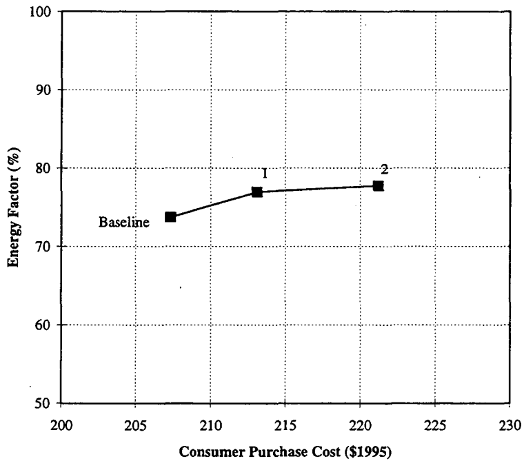
Figure 11.4. Cost Versus Efficiency for New Electric Cooktops with a Coil Element
