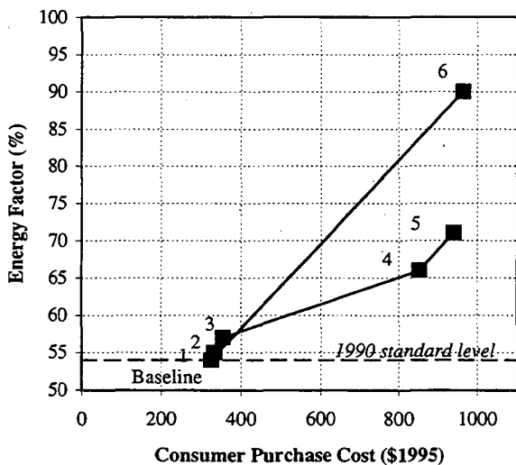
Figure 4.6. Cost Versus Efficiency for New Gas Storage Water Heater
