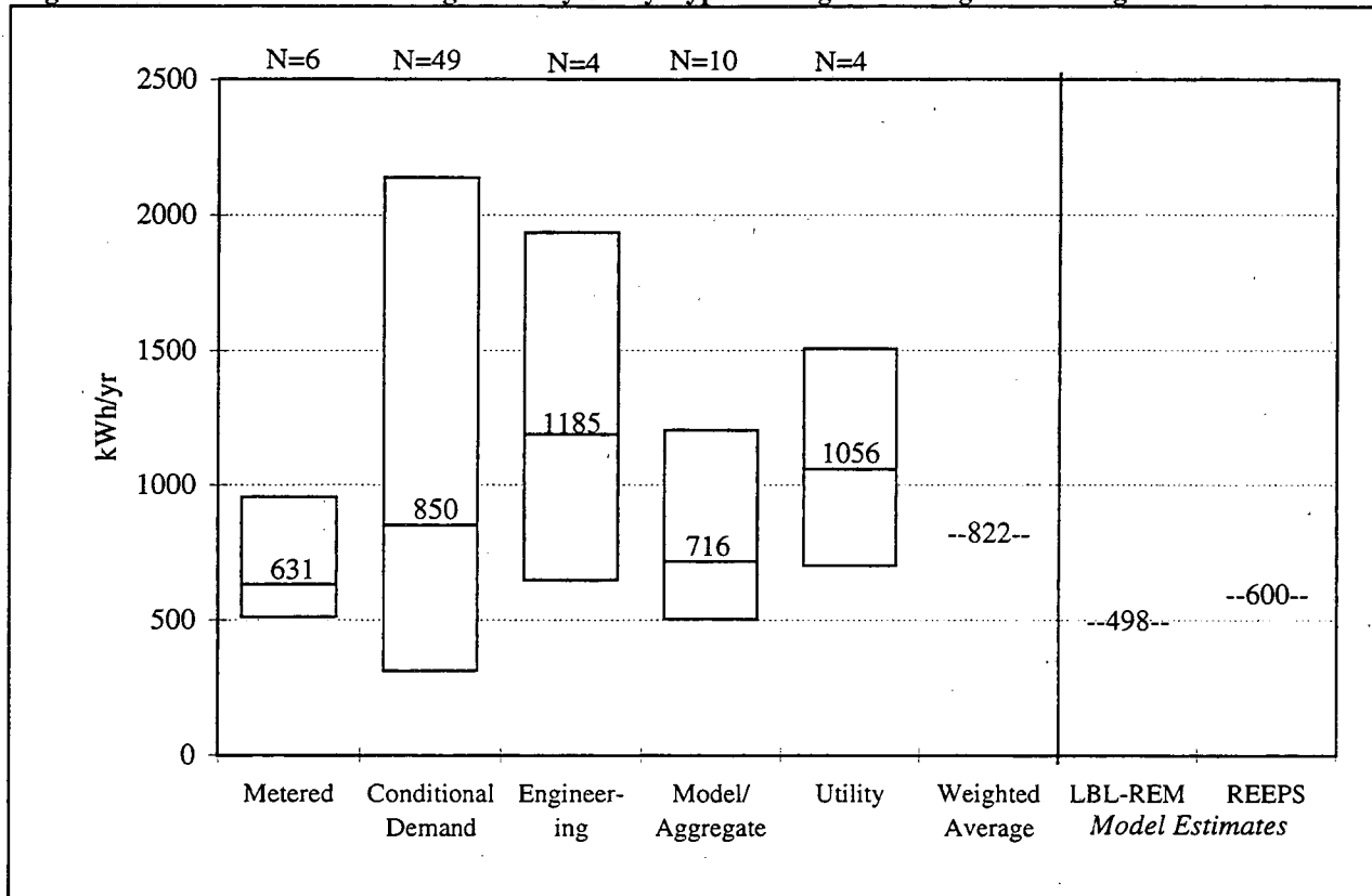
Figure A.4. Electric Cooking UECs by Study Type -- Range and Weighted Average
