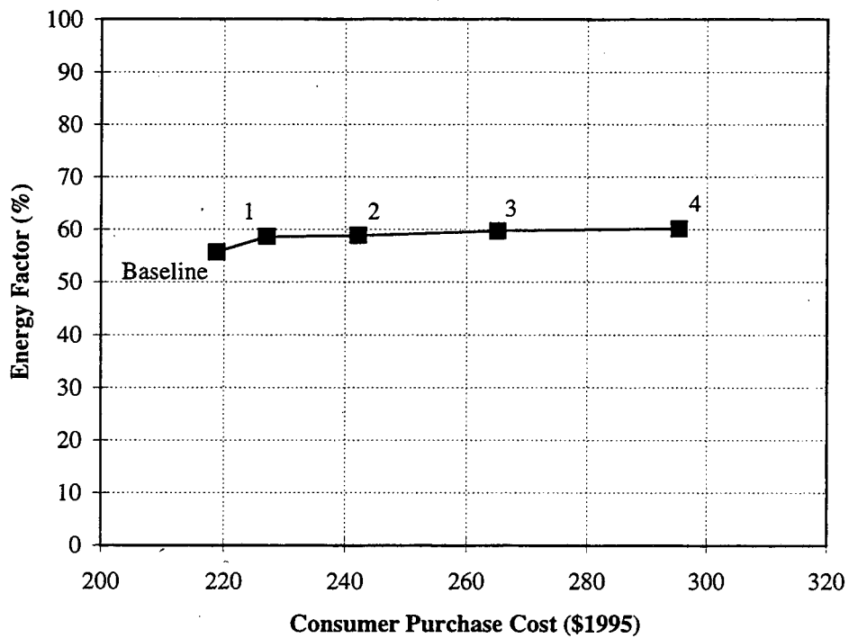
Figure 11.10 Cost Versus Efficiency for New Microwave Ovens
