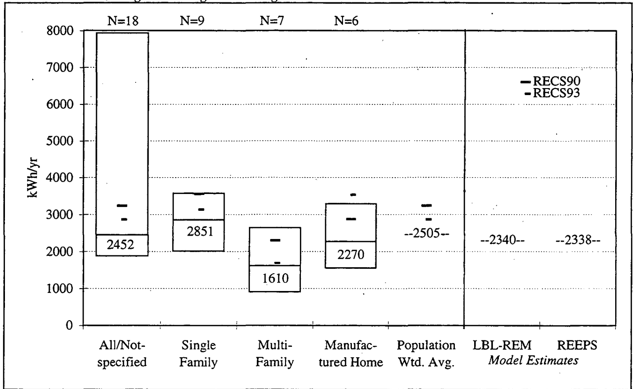
Figure A.8. National Average Central Air Conditioner UECs by House Type Range and Weighted Average
