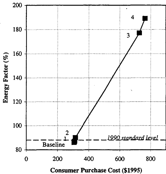
Figure 4.5. Cost Versus Efficiency for New Electric Storage Water Heater
