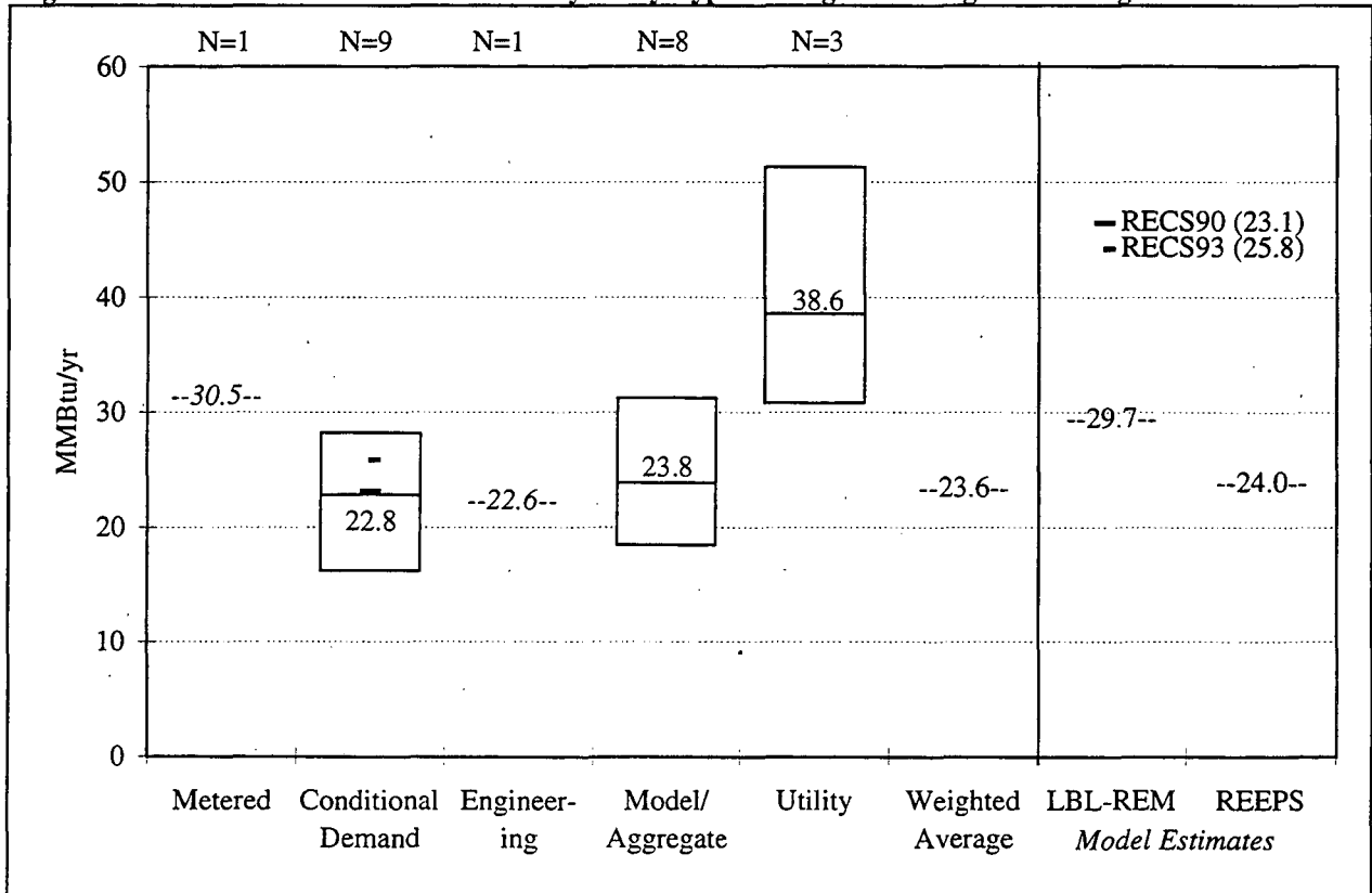
Figure A.7. Gas Water Heater UECs by Study Type -- Range and Weighted Average
