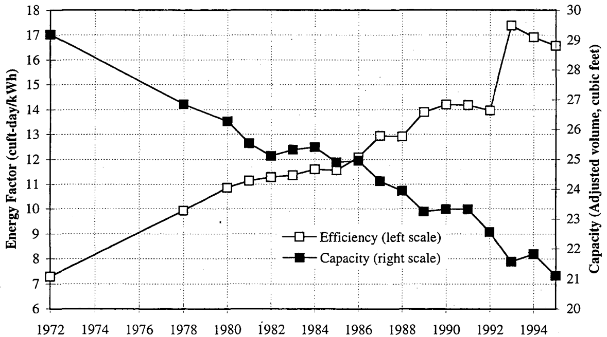
Figure 6.2. Shipment-Weighted Energy Factor and Capacity for Freezers, 1972-1995
