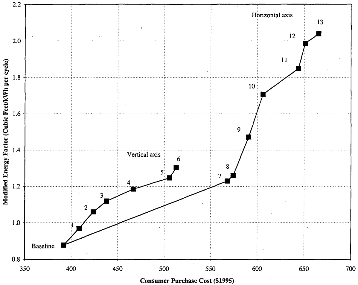
Figure 8.3. Cost Versus Efficiency for New Clothes Washer
