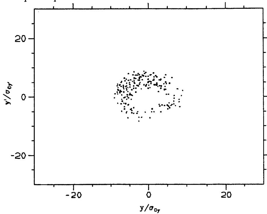
Figure 9(b). The vertical distribution of the injected beam in normalized phase space after 8000 turns.
