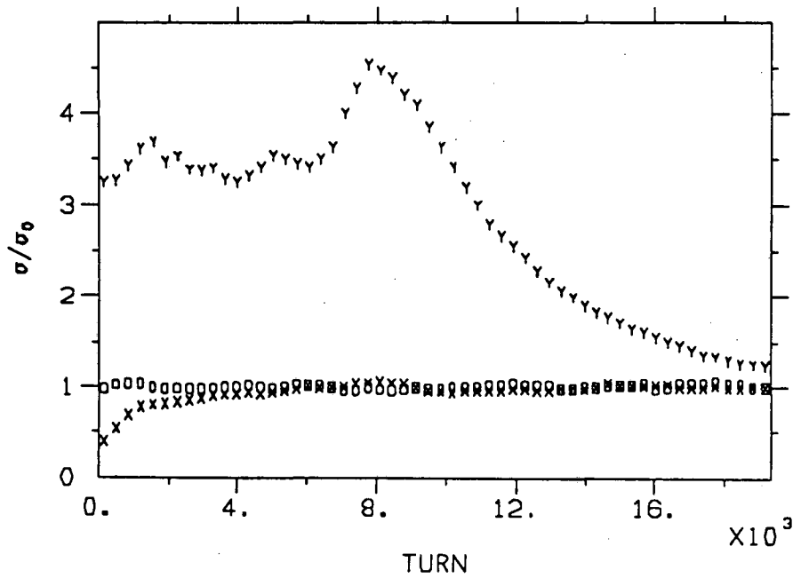
Figure 7. The time evolution of the injected beam sizes in units of the nominal storage ring beam sizes during the vertical injection process (x=horizontal, y=vertical, and o=longitudinal).
