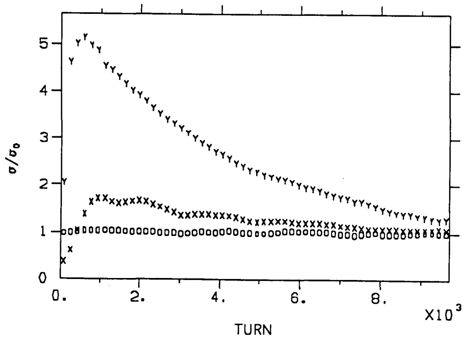
Figure 10(b). The time evolution of the normalized sizes of the injected beam for the vertical separation d_y = 6\sigma_{0x,+} .
