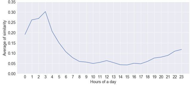
Figure 3.11: The relation between average similarity matrix and the hours of a day.
