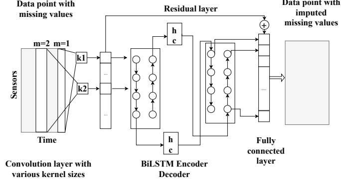
Figure 4.3: A convolutional BiLSTM encoder decoder (CNN-BiLSTM-Res) for missing data imputation
