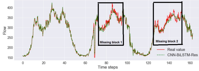
Figure 4.7: The illustration of missing data imputation for one sensor by the proposed model
