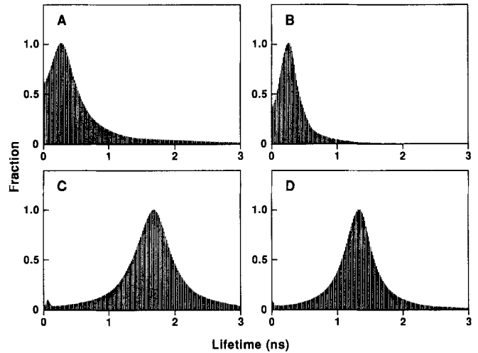
Figure 3. Lorentzian lifetime distributions for the Chl a fluorescence decay in pea thylakoid membranes (A and C) and core PSII (B and D) in the presence of 5 \mu M DCMU (C and D: Q_A^- -closed PSII centers) and 15 \mu M DCBQ (A and B: open PSII centers). The open center data were fitted with a single Lorentzian function, and the Q_A^- -closed center data were fitted with a double Lorentzian function. The other details are given in the legend of Fig. 1.
