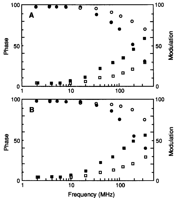
Figure 1. Phase (in degrees; squares) and modulation (full scale, 100%; circles) as a function of frequency for the Chl a fluorescence decay in pea thylakoid membranes (A) and core PSII (B) in the presence of 5 \mu M DCMU (closed symbols) ( Q_A^- -closed PSII centers) and 15 \mu M DCBQ (open symbols) (open PSII centers). Samples were suspended in a reaction medium containing 0.4 M sorbitol, 5 mM MES-KOH (pH 6.5), 20 mM KCl, 2 mM MgCl 2 and 1 \mu M nigericin. The Chl concentration was 5 \mu M .
