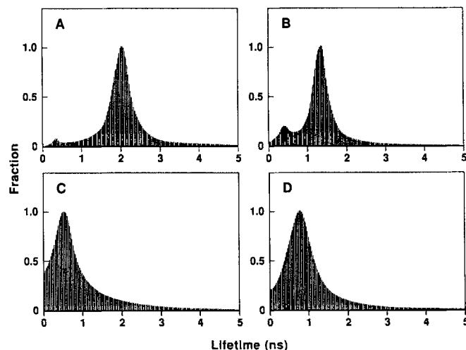
Figure 5. Lifetime distribution for Chl a fluorescence decay in spinach thylakoid membranes (A and C) and PSII membranes (B and D) in the presence of laser illumination for the Q_A^- -closed centers (A, B) and sodium dithionite and methyl viologen plus laser light for doubly reduced Q_A (C, D); also see legend for Fig. 4 and Materials and Methods. Data were best fit with double and single Lorentzian functions, respectively.
