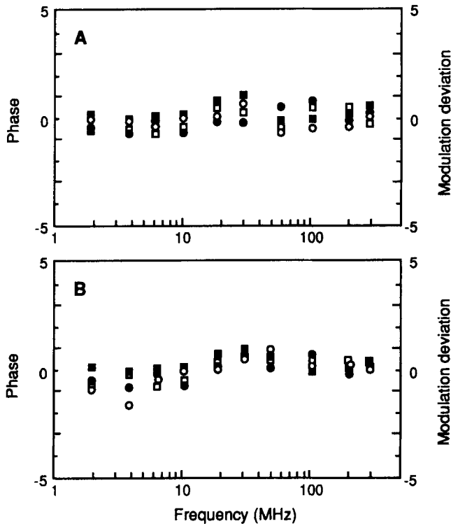
Figure 2. Phase (in degrees; squares) and modulation (with full scale as 100%; circles) deviations given as weighted residuals between the calculated and experimental data of Fig. 1 are shown in the middle of the plot with scale +5 to -5. (A): pea thylakoid membranes. (B): core PSII. All symbols are as described in the legend of Fig. 1. The nonlinear least-squares data analysis procedure was applied.
