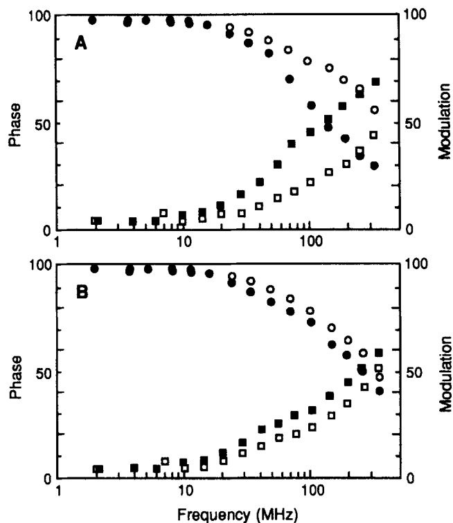
Figure 4. Phase (in degrees; squares) and modulation (full scale, 100%; circles) as a function of frequency for the Chl a fluorescence decay in spinach thylakoid membranes (A) and PSII membranes (B) of Q_A^- -closed centers (closed symbols) and of doubly reduced Q_A centers (open symbols). See Materials and Methods. Illumination after treatment with dithionite and methyl viologen was done with a standard flashlight and subsequently with 1.5 W 532 nm laser light for 2 min. The Q_A^- -closed centers were generated simply by illumination with the laser.
