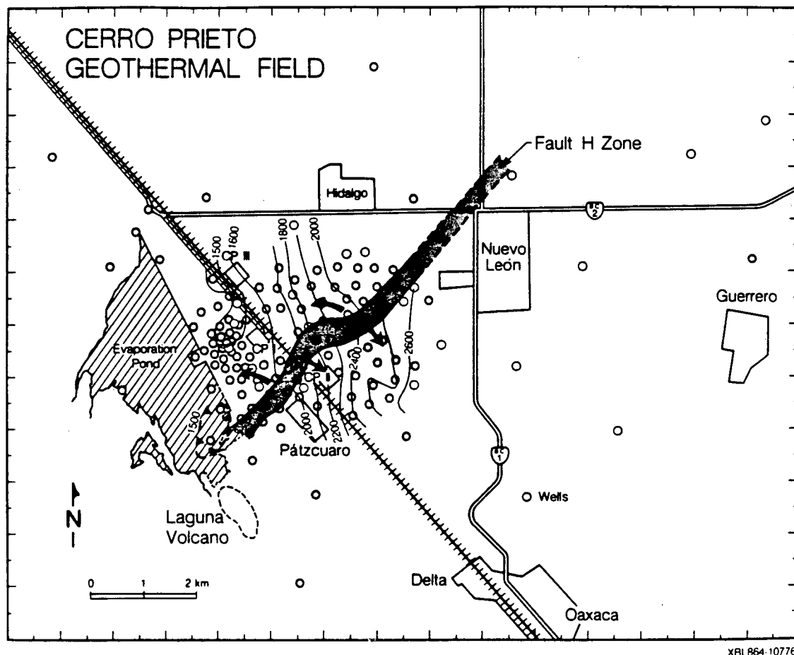
Figure 8. Depth (in meters) to the top of the Sand Unit Z. The arrows indicate the direction of geothermal fluid flow away from the Fault H zone into the \beta reservoir. The fault is shown at the \beta reservoir level.
