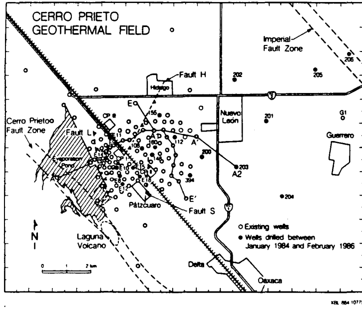
Figure 2. Location of old and new wells, principal faults, and cross sections A-A', A1-A2, and E-E'. The faults are projected to the surface.
