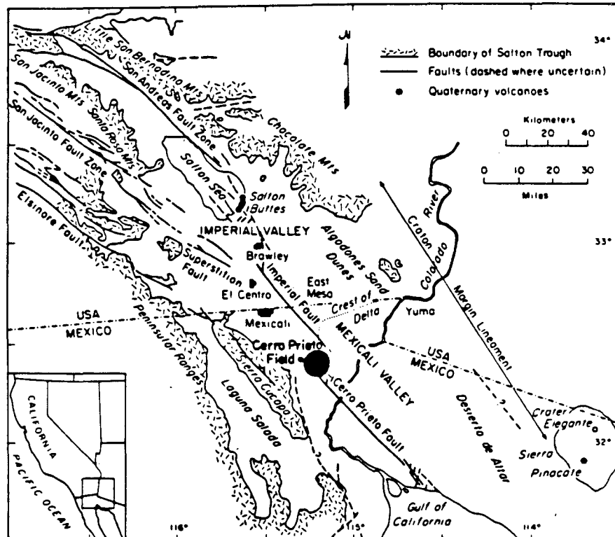
Figure 1. Location of the Cerro Prieto field in the Salton Trough, that includes the Imperial and Mexicali Valleys.
