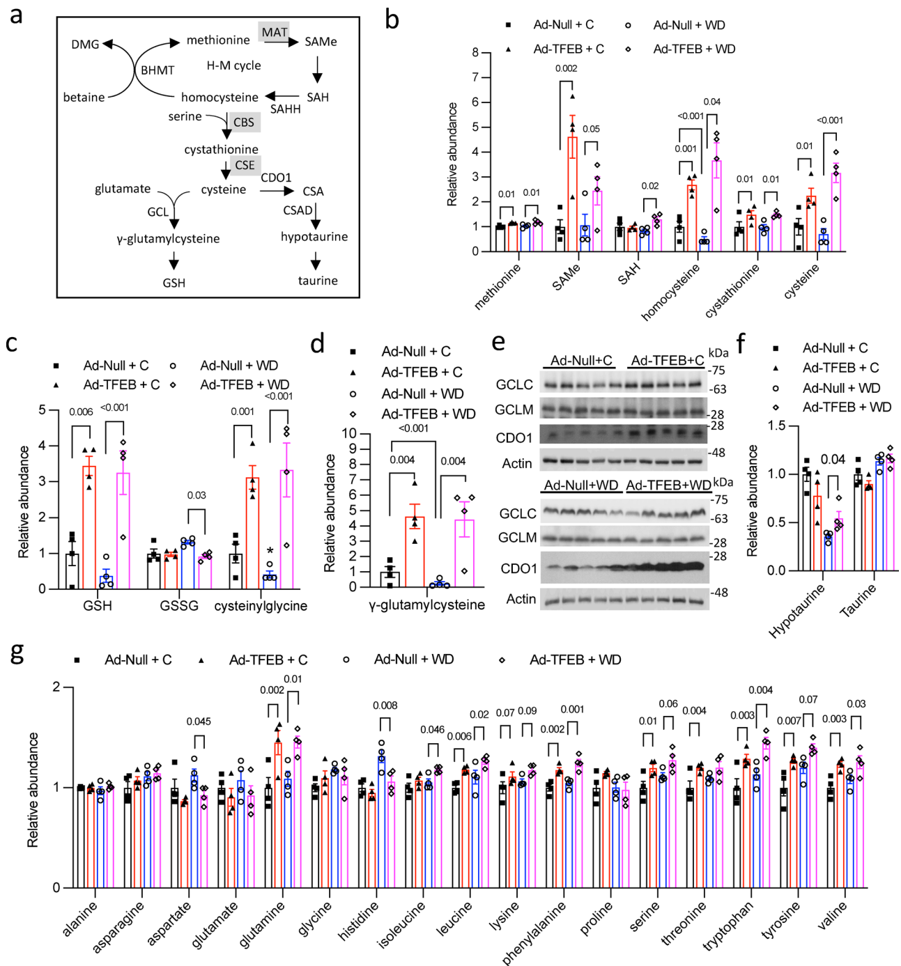
Fig. 2 | TFEB stimulates methionine cycle-transsulfuration to increase hepatic cysteine and GSH pool. a Illustration of methionine cycle-transsulfuration pathway and GSH and taurine synthesis. MAT1A Methionine adenosyltransferase 1A, CBS cystathionine β-synthase, CSE cystathionine γ lyase, SAMe S-adenosylmethionine, SAH S-adenosylhomocysteine, BHMT betaine-homocysteine S-methyltransferase, CDO1 cysteine dioxygenase 1, CSAD cysteine sulfinic acid decarboxylase, GCL glutamate cysteine ligase, GCLC glutamate cysteine ligase catalytic subunit, GCLM glutamate cysteine ligase modifier subunit, CSA cysteine sulfinic acid, H-M cycle homocysteine–methionine cycle, DMG dimethylglycine. GSH: reduced glutathione. b, c, d Male 10 weeks old C57BL/6J mice were intravenously injected with Ad-Null or Ad-TFEB at 5 \times 10^8 pfu/mouse. One week later, mice were
