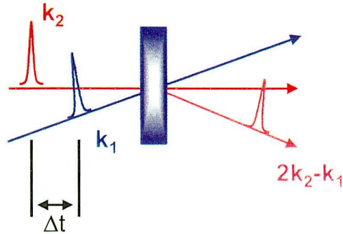
Figure 2.1: FWM emission.
