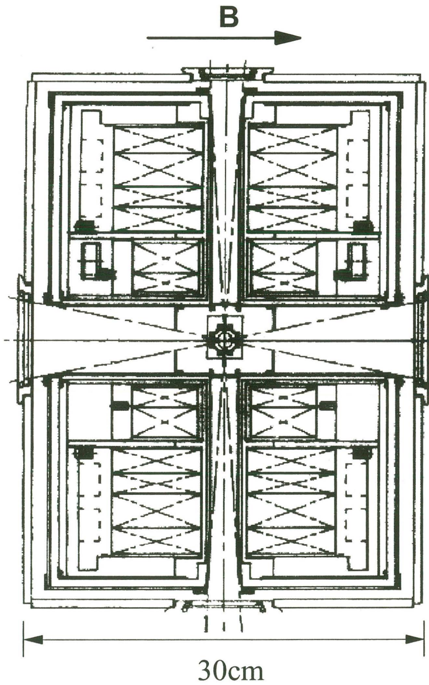
Figure 3.5: Magnet cross-section. The angular aperture is 25.5°.
