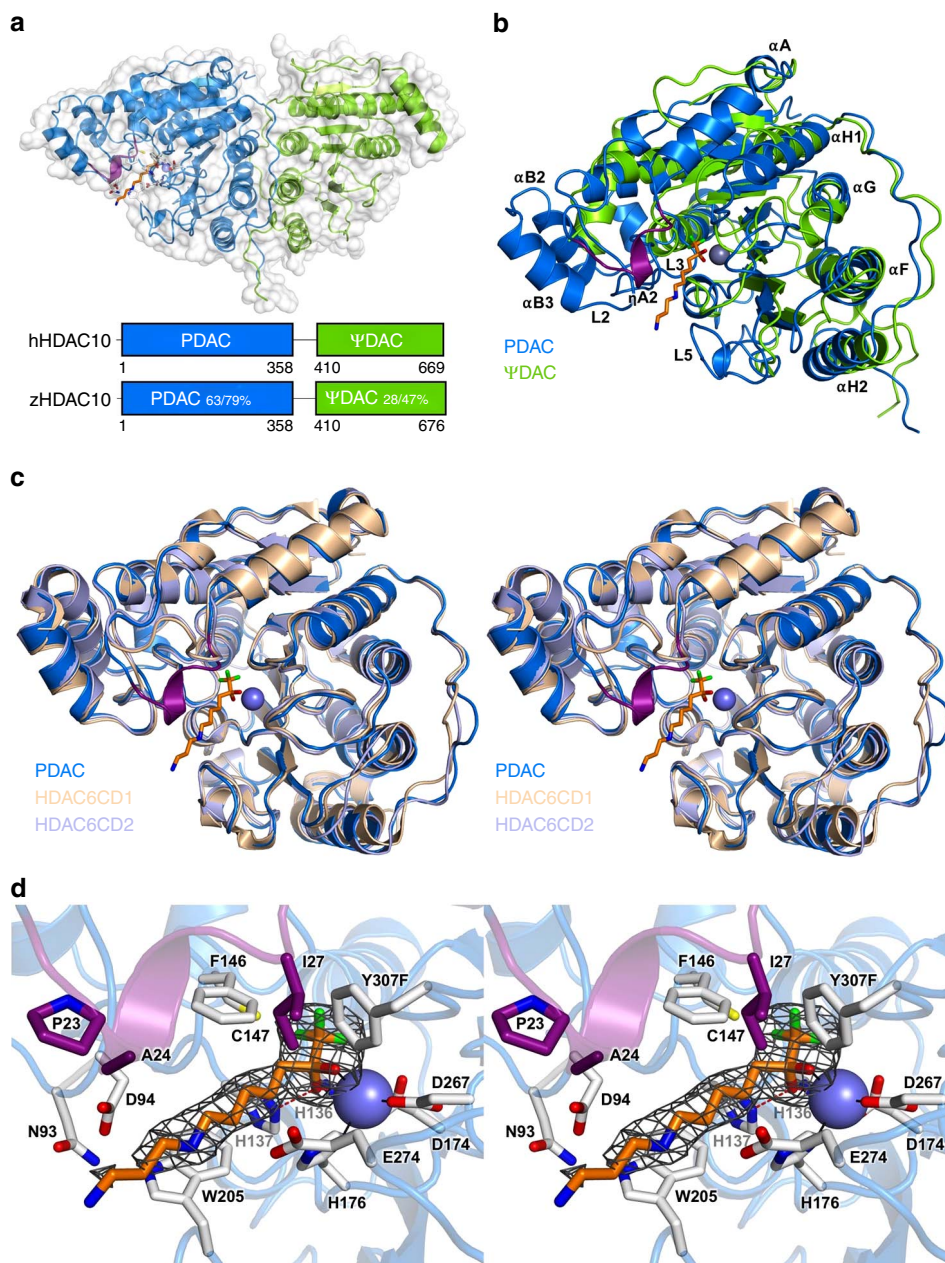
Figure 3 | Crystal structure of the Y307F zHDAC10 \Delta -AAT complex. (a) The catalytic PDAC domain and the smaller, noncatalytic \Psi DAC domain assemble with butterfly-like architecture. The unique 3_{10} -helix \eta A2 (P 23 ACE) found in the L1 loop of HDAC10 orthologues is purple. Percentages indicate sequence identity/similarity between zebrafish and human HDAC10 domains. The inhibitor AAT (stick figure, C = yellow, N = blue) binds to the PDAC domain. (b) Superposition of the PDAC domain (blue) with the \Psi DAC domain (green). Selected secondary structure elements are labelled: helix \eta A2 is purple; helices \alpha F, \alpha G and the loop connecting helices \alpha H1 and \alpha H2 mediate domain-domain interactions; helices \alpha B2 and \alpha B3, as well as loops L1-L5, comprise and flank the active site of PDAC but are absent in \Psi DAC (for clarity, only loops L2, L3 and L5 are labelled). Zn^{2+} is a blue sphere. (c) Stereo view image showing the superposition of zHDAC10 PDAC domain (blue), zHDAC6 CD1 (wheat, PDB 5EEF) and zHDAC6 CD2 (light blue, PDB 5EFH). The 3_{10} -helix \eta A2 inserted in loop L1 (purple) is unique to zHDAC10 and serves to constrict the PDAC active site. (d) Stereo view image showing the simulated annealing omit map of AAT bound in the PDAC active site contoured at 3\sigma . Selected active site residues are indicated; hydrogen bonds are indicated by dashed red lines and metal coordination interactions are represented by solid black lines. Zn^{2+} is a blue sphere.
