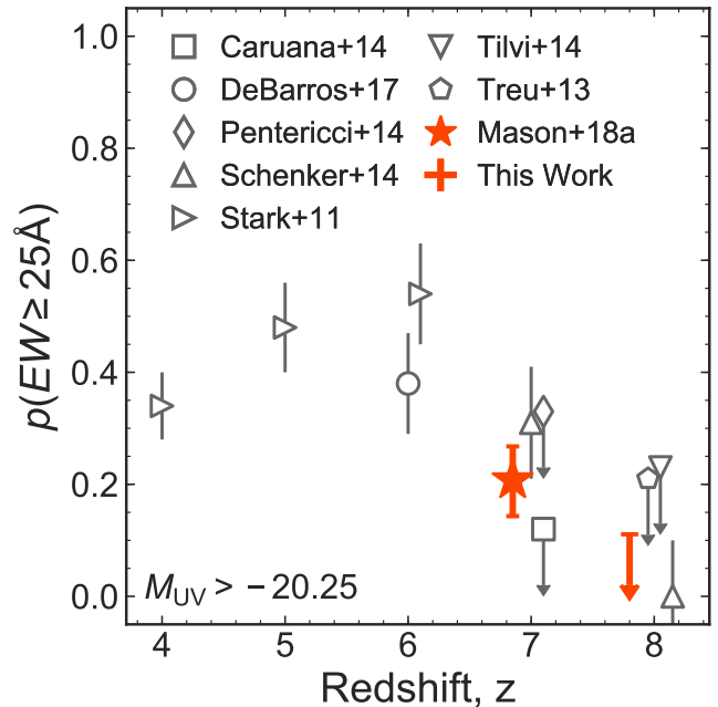
Figure 7. The redshift evolution of the ‘Ly \alpha fraction’ for UV faint galaxies, the fraction of LBGs observed with Ly \alpha EW \geq 25 \text{\AA} . We plot literature measurements from Stark et al. (2011); Pentericci et al. (2014); Treu et al. (2013); Tilvi et al. (2014); Schenker et al. (2014); Caruana et al. (2014) and De Barros et al. (2017). We add small offsets in redshift for measurements at the same redshifts to ease the display of the data. We also plot the predicted Ly \alpha fraction from M18a calculating p(W > 25 | \bar{x}_{\text{HI}}, M_{\text{UV}}) using M_{\text{UV}} = -20 galaxies and the neutral fraction constraint \bar{x}_{\text{HI}} = 0.59^{+0.11}_{-0.15} (16 – 84% confidence intervals) as the orange star. We plot the upper limits recovered in this paper as orange lines, with the solid line showing our 68% confidence limit, and the dotted line extending to the 95% confidence limit. We calculate p(W > 25 | \bar{x}_{\text{HI}} > 0.76, M_{\text{UV}}) again using M_{\text{UV}} = -20 . Our constraint is consistent with literature values at the same redshift.
