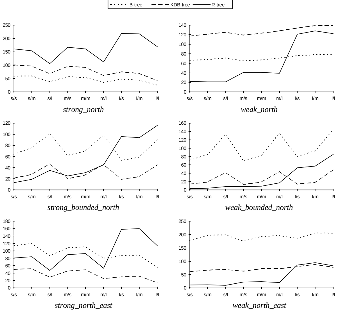
Fig. 10 Performance Comparison (disk accesses per data/query size combination)
