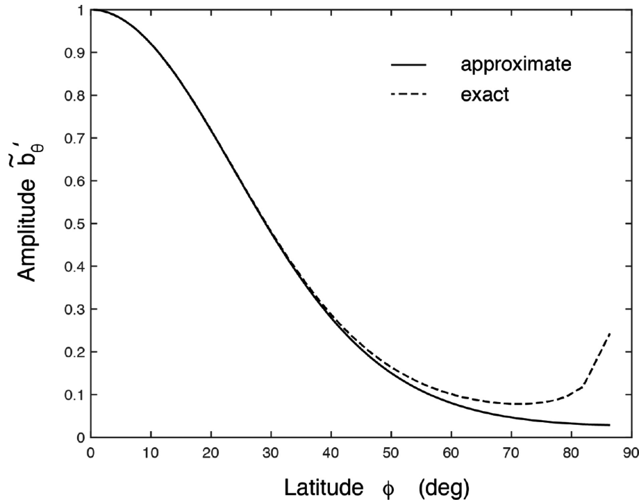
Figure 6. Amplitude of low-frequency eMAC waves computed using a constant M on the extended beta-plane. The eigenfunction, \tilde{b}'_{\theta} , is computed from \tilde{b}''_{\theta} using the approximate (solid) and exact (dashed) transformation. Errors near the north pole arise when the exact transformation is used with an incomplete description of the spherical geometry on the extended beta-plane. These errors are reduced by using the approximate transformation. There is little difference in the structure of the wave near the equator.
