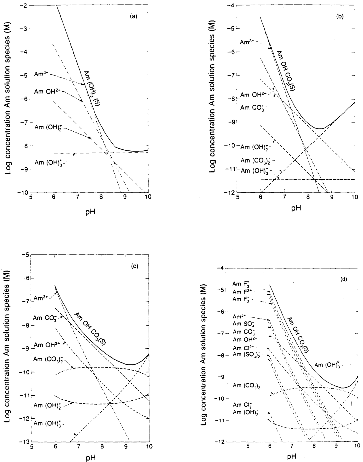
Fig. 1. Calculated concentrations of Am solution species (dashed curves-labelled with species) and their sums (solid curves-labelled with the controlling solid phase) for 0.1 M ionic strength as a function of pH. (a) P(\text{CO}_2) = 0 atmos.; (b) P(\text{CO}_2) = 10^{-3.5} atmos.; (c) \Sigma \text{CO}_3 = 2 \times 10^{-3} M; (d) simulated ground water of low dissolved solids: \text{Cl}^- = 8.4 \times 10^{-3} M, \text{SO}_4^{2-} = 2.1 \times 10^{-3} M, \text{F}^- = 2.2 \times 10^{-3} M, \Sigma \text{CO}_3 = 2.6 \times 10^{-3} M.
