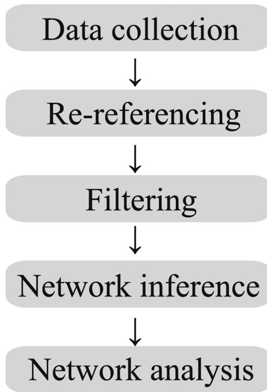
Figure 1: A candidate functional network analysis pipeline, with five steps. While the arrows indicate a linear progression between steps, the interactions between steps are more complicated.
