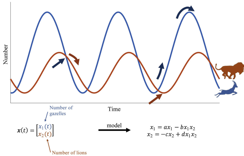
Figure 3: Predator-prey model (Top) Population of lions and gazelles over time. (Bottom) Dynamical 2-node network model describing populations over time, assigning a differential equation for each population.
