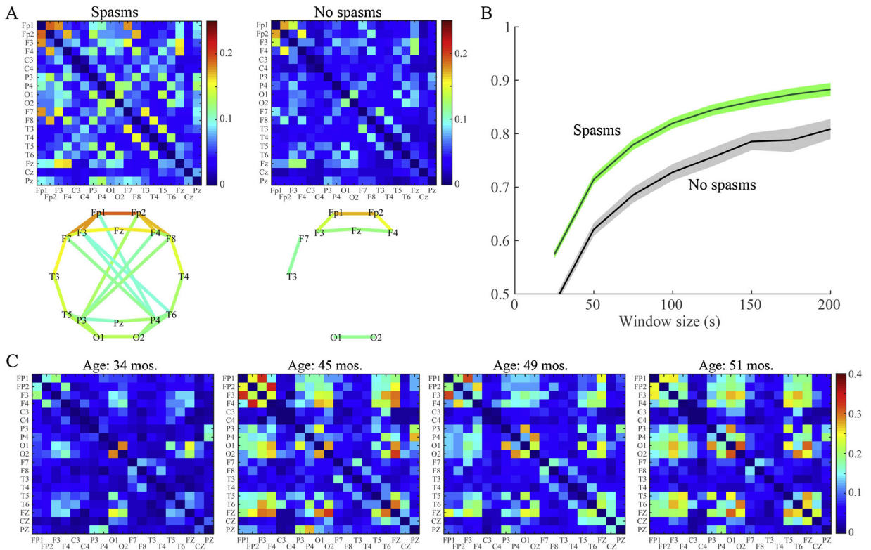
Figure 6: Epileptic spasms are associated with strong, stable functional networks. (A) Average functional connectivity matrices (top row) and network maps (bottom row) for patients with and without spasms. The color represents the connectivity strength, defined as the proportion of 1-second epochs for which the connectivity between two channels was statistically significant. Network maps show all connections with strength > 0.1. (B) Test-retest reliability of the FCN for the spasms group (green) and the non-spasms group (gray) measured via 2D correlation of the connectivity matrices for EEG segments of varying length. The solid lines represent the mean, and shaded areas denote the 95% confidence interval across all subjects in the group. FCNs are reliable when measured using segments of EEG at least 150 seconds long, and the spasms group exhibited higher reliability than controls. (C) A representative example of FCNs from longitudinal EEGs of a patient who had spasms and was diagnosed with Lennox-Gastaut at 45 months old. The strength of the FCN increases with onset of Lennox-Gastaut and varies over time; however, note that the locations of the strongest connections in the network remain stable over the 17 month period. This patient experienced continued seizures, despite multiple medication changes.
