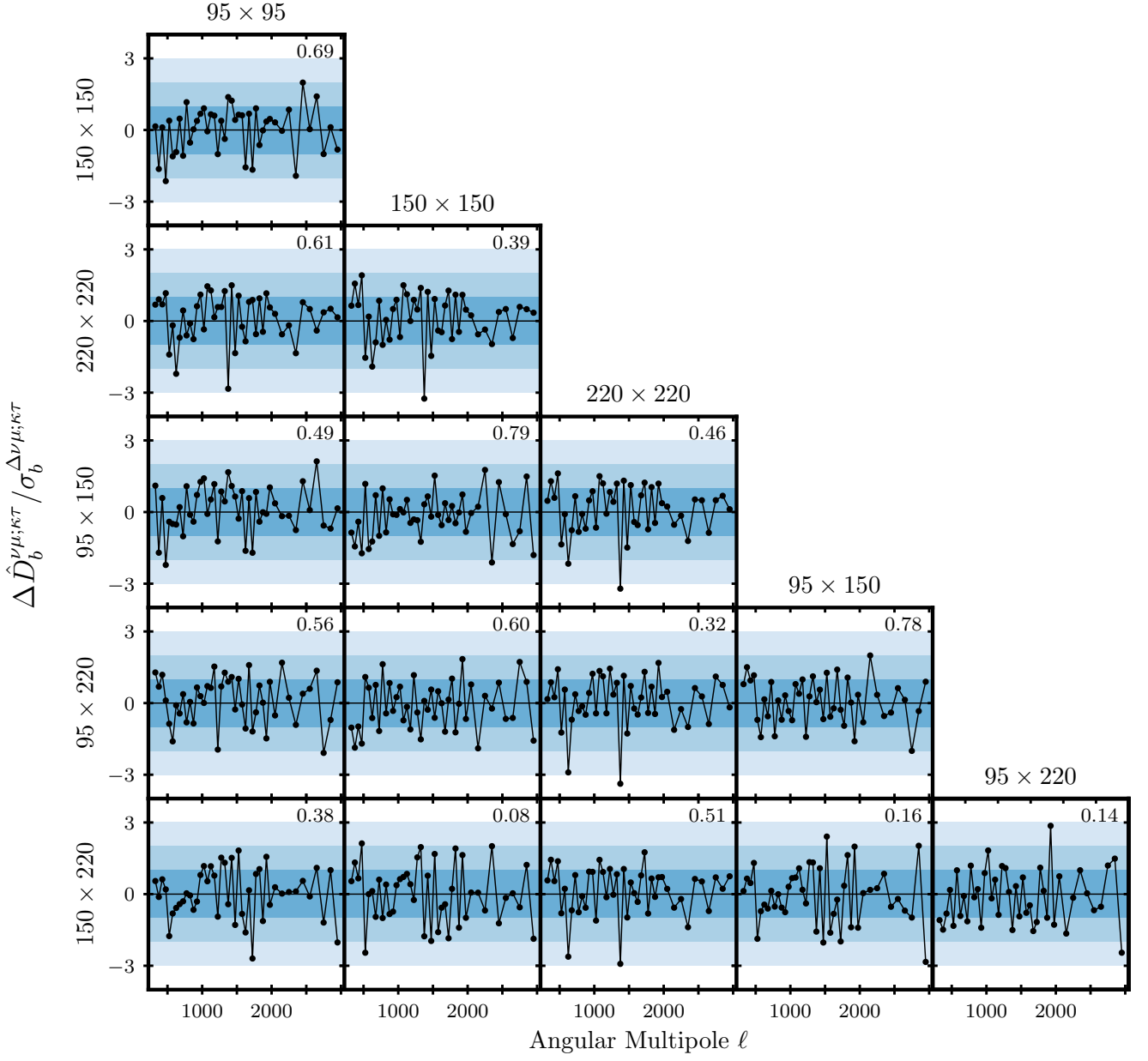
FIG. 16. Relative EE difference spectra as indicated by the row and column labels, i.e. difference spectra \Delta\hat{D}_b^{\nu\mu;\kappa\tau} divided by the square root of the associated covariance, \sigma_b^{\Delta\nu\mu;\kappa\tau} . The blue shading indicates the range of 1 - 3\sigma fluctuations. The multifrequency spectra are in good agreement with one another, as evidenced by the PTE values (given in the top right corner of each panel) which all lie in the 95th percentile.
