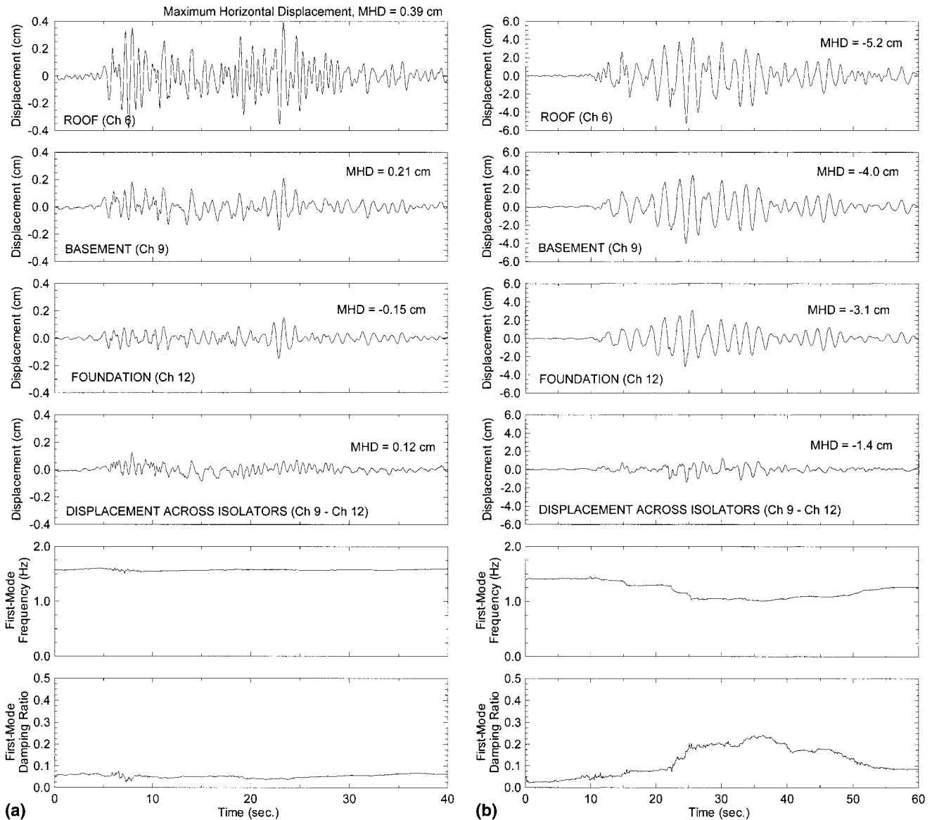
FIG. 1. Displacement Time Histories and Time Variation of First-Mode Parameters: (a) FCLJC, 1987 Whittier Earthquake (Transverse, NS Direction); (b) FCLJC, 1992 Landers Earthquake (Transverse, NS Direction)
