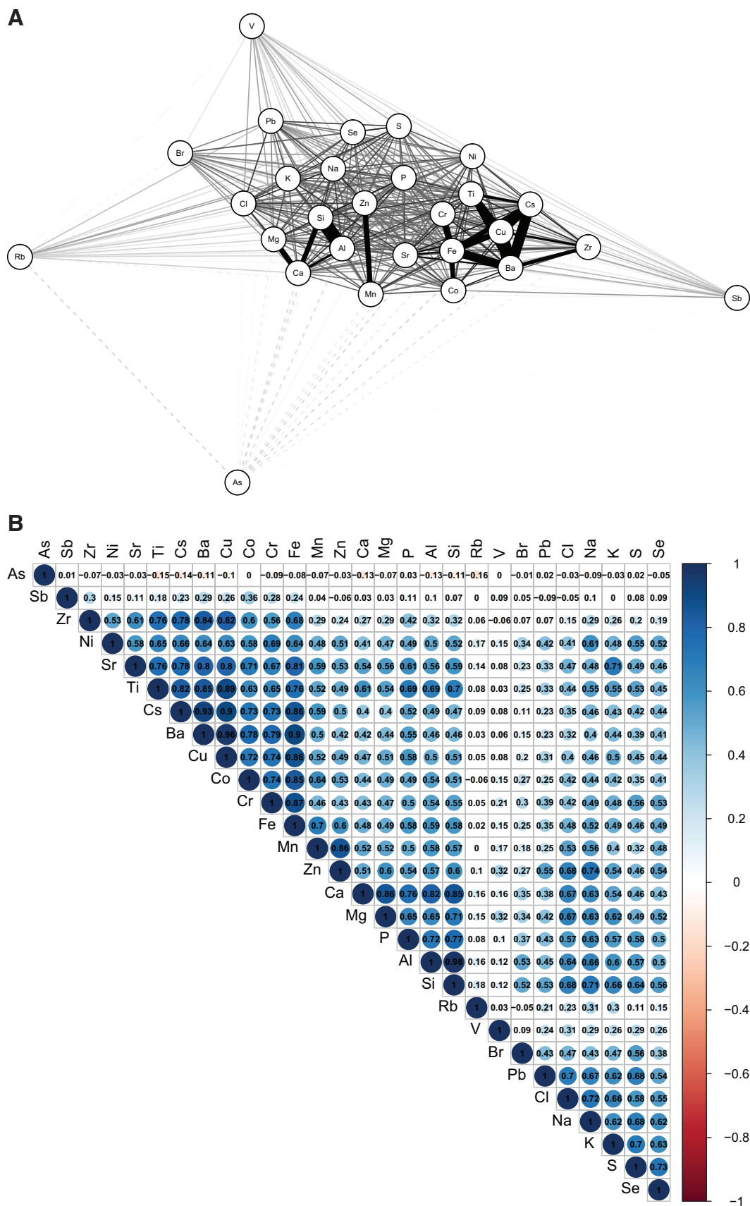
Figure 1. Correlations between PM 2.5 metals during summer. A, Network plot with more highly correlated metals grouped more closely together and linked by darker, thicker lines (dashed lines indicate inverse correlations). Numeric correlation values are illustrated in B.
