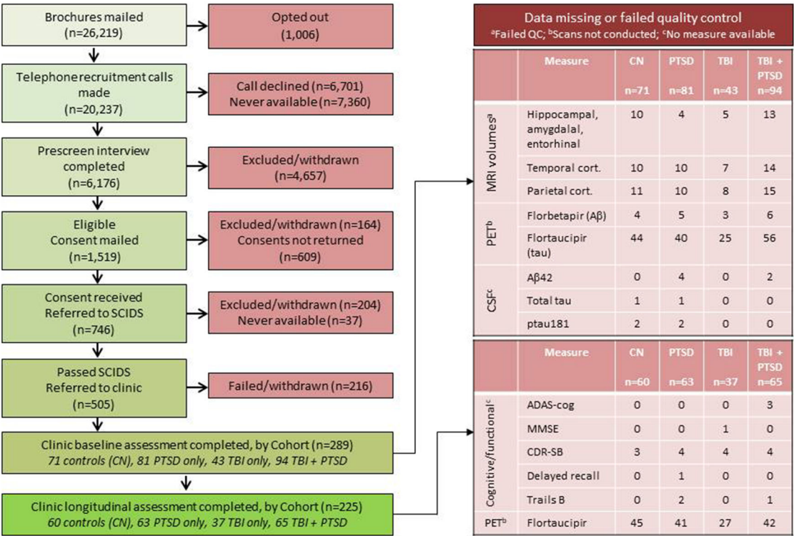
Figure 1. Flow of DOD ADNI recruitment and enrollment. Abbreviations: ADAS-cog; Alzheimer’s Disease Assessment Scale – cognitive; CDR-SB, Clinical Dementia Rating – Sum of Boxes; CN, control; cort., cortical; CSF, cerebrospinal fluid; MMSE, Mini-Mental State Examination; MRI, magnetic resonance imaging; PET, positron emission tomography; PTSD, posttraumatic stress disorder; SCIDS, Structured Clinical Interview for DSM; TBI, traumatic brain injury.
