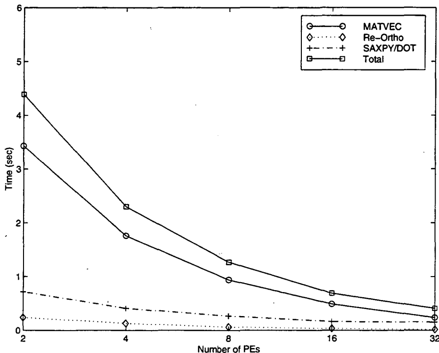
Figure 2: Time to compute the five largest eigenvalues of NASASRB with different number of processors.
