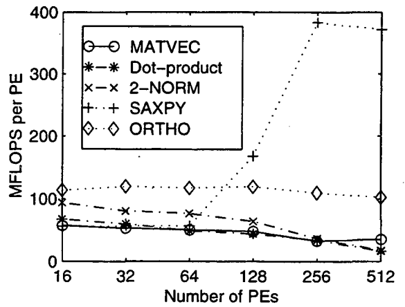
Figure 1: Scalability of core operations of PLANSO on T3E with fixed global problem size.
