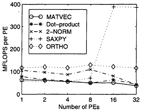
Figure 1: Scalability of core operations of PLANSO on T3E with fixed global problem size.
