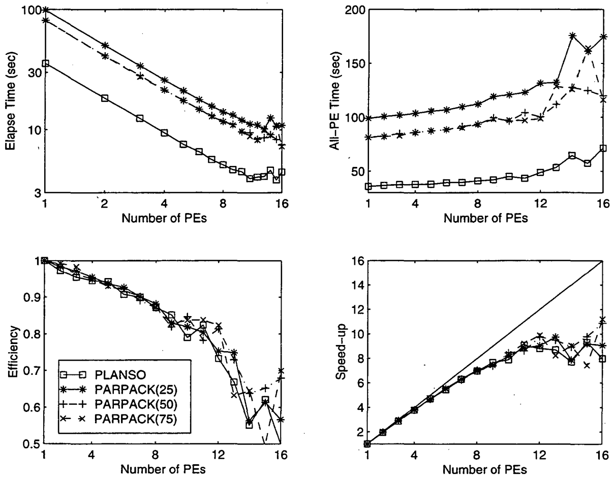
Figure 9: Performance of PLANSO and PARMACK on a cluster of 2 8-PE SPARC Ultra workstations.
