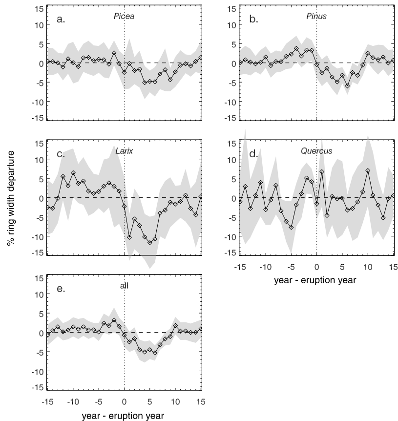
Figure 4. Mean ring width departures around eruption years among sites north of 45^{\circ} N, for (a–d) the most common tree genera in the database and (e) the mean of all sites north of 45^{\circ} N. Shading shows 2-standard error confidence limits based on the variation across eruption years. See Table 2 for number of sites and significance levels of departures for each group. Table 1 lists the eruption years used.
