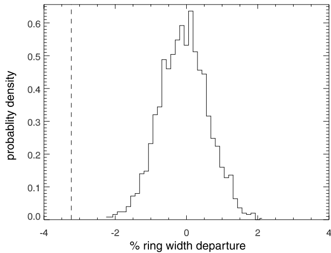
Figure 3. An example of the Monte Carlo analysis used to test regional width departures for significance: width departure for sites north of 45^{\circ} N for years 0–8 following eruption years (dashed line) as compared to the distribution of mean widths from the same sites following 1000 sets of random “eruption years” (histogram). Here the negative departure is significant, p < 0.001 .
