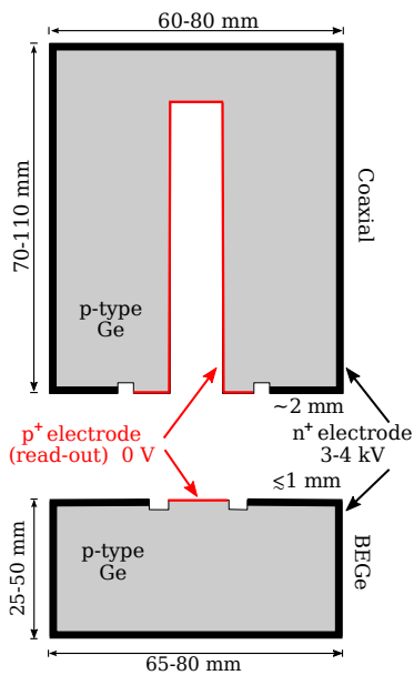
Fig. 1 Schematic sketch of a coaxial HPGe detector (top) and a BEGe detector (bottom) with their different surfaces and dead layers (drawings not to scale), adapted from Ref. [25].
