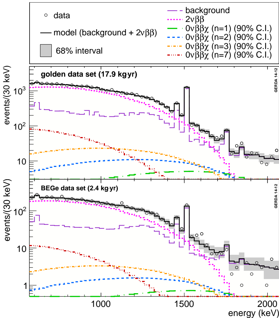
Fig. 3 Best-fit model and data energy spectrum for the coaxial and the BEGe data sets for the case of spectral index n = 1 . The contributions from 2\nu\beta\beta decay and the background contributions are shown separately. The best-fit model does not contain the contributions from 0\nu\beta\beta\chi . The smallest interval of 68% probability for the model expectation is indicated in grey. Also shown is the upper limit for 0\nu\beta\beta\chi decay with n = 1 as determined from the 90% quantile of the marginalized posterior probability for 1/T_{1/2}^{0\nu\chi} . For illustrative purpose, also the upper limits at 90% C.I. of the other three spectral indices n = 2, 3, 7 are reported.
