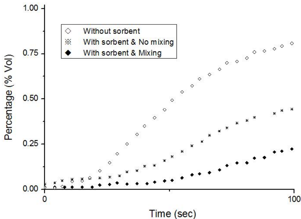
Fig.3.17 The evolution of CO 2 with different feedstock-sorbent contact type
