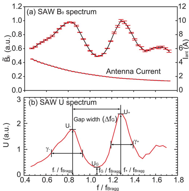
FIG. 6. (Color online) Two different representations of the SAW spectrum at port 14 with the baseline mirror configuration ( M=0.25 ). (a) Normalized \vec{B}_\theta vs f/f_{\text{Bragg}} ; antenna current rms value is also overplotted (error bars may be too small to be distinguished from the curve); (b) “disk energy density” normalized using a constant ( 1.0 \times 10^5 / \mu_0 \pi ) vs f/f_{\text{Bragg}} . f_{\text{Bragg}} = 160 kHz. (All data acquired with 100 MHz sampling rate, averaging eight samples and five consecutive plasma shots. Maximum horizontal error is \pm 0.01 .)
