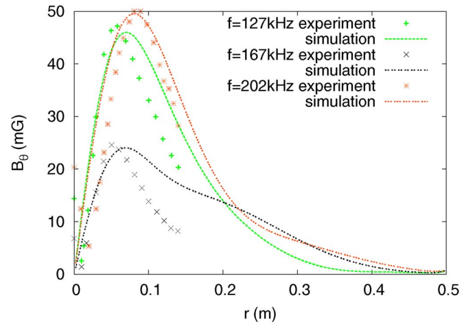
FIG. 14. (Color online) The radial profiles of azimuthal B field (rms) at three frequencies comparing simulation and experiment results. This simulation uses \alpha = 4 which is defined in Eq. (26).
