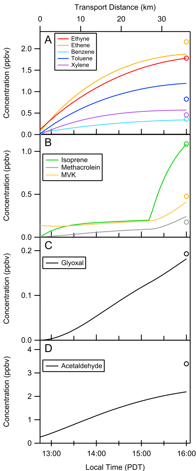
Figure 3. Results from the Master Chemical Mechanism v3.2 “base case” model. These results are presented numerically in Table 2. VOC concentrations are plotted for an air parcel that starts at the coast (time = 12:45 PDT; distance = 0 km) and arrives at the CalNex ground site (time = 16:00 PDT; distance = 37 km). (a) Modeled anthropogenic concentrations for ethyne, ethene, benzene, toluene, and xylenes as a function of transport time. Average values measured at the CalNex ground site at 16:00 PDT are shown as open circles. (b) Modeled biogenic concentrations for isoprene and its oxidation products methacrolein and MVK. Average values measured at the CalNex ground site at 16:00 PDT are shown as open circles. (c) Modeled glyoxal concentrations as a function of transport time. Average value measured at the CalNex ground site at 16:00 PDT is shown as an open circle. (d) Modeled acetaldehyde concentrations as a function of transport time. Average value measured at the CalNex ground site at 16:00 PDT is shown as an open circle.
