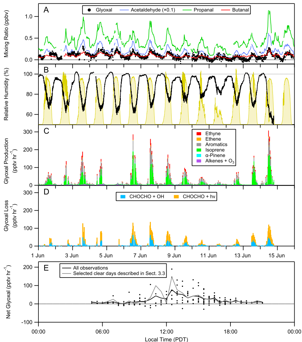
Figure 2. (a) Time series of aldehydes during 1 June to 16 June 2010 showing glyoxal, acetaldehyde, propanal, and butanal. Plotted glyoxal data are 10 min averages. Other aldehydes are measured for 5 min every 30 min. (b) Time series of measured relative humidity and j_{NO_2} (yellow bars; units not shown). (c) Time series of the glyoxal production rate calculated from measured VOC, OH, and O 3 concentrations, showing ethyne, ethene, aromatics, isoprene, \alpha -pinene, and alkenes + O 3 . (d) Time series of the glyoxal loss rate calculated from CHOCHO + OH and CHOCHO + hv. (e) Net glyoxal calculated from the difference between production (Figure 2c) and loss (Figure 2d), calculated for all observations and for selected dates used in the MCM analysis. Data are shown as a diurnal average.
