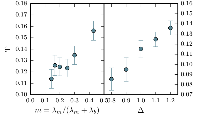
FIG. 5. The threshold temperatures as a function of measurement fraction, m (left), and the Hamiltonian energy scale \Delta (see Eq. 1)(right). At zero measurement fraction, the critical temperature is 0, and at unit measurement fraction, the critical temperature is \mathcal{O}(1) .
