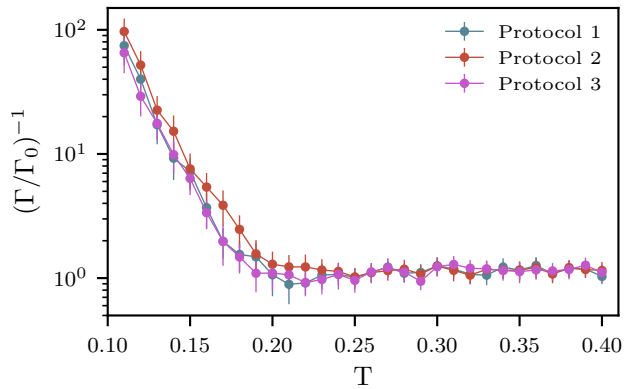
FIG. 7. Comparison of three different functional forms used as proxies for P(d_1 : d_2) . Protocol 1 is simply the error function expression given by Eq. 12. Protocol 2 is the probability density \frac{1}{2\pi D|t_2 - t_1|} \exp(-\frac{|x_2 - x_1|^2}{2D|t_2 - t_1|}) . Protocol 3 is the more complicated expression in the last line of Eq. A2. In practice, each approximation for P(d_1 : d_2) is seen to perform approximately equally well.
