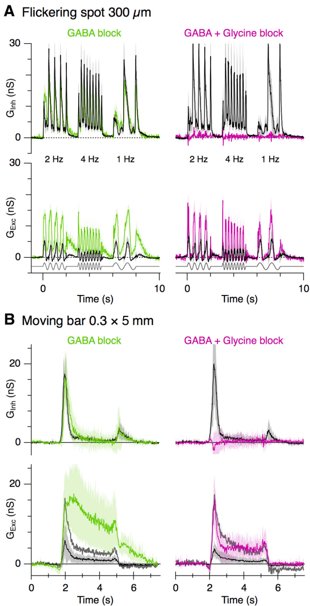
Figure 6. Inhibitory synaptic inputs to ON-DSGCs comprise direct glycinergic inputs. A , Average inhibitory and excitatory conductances recorded in control (black) and during application of 10 \mu\text{M} SR95531 + 10 \mu\text{M} TPMPA (GABA block, green; n = 5 ). Top row shows inhibition; bottom row shows excitation. Sinusoidal flicker frequency indicated beneath. Three recordings remained stable enough for the subsequent addition of 1 \mu\text{M} strychnine (GABA + Glycine block, magenta; n = 3 ). Centered light spot, 300 \mu\text{m} diameter, 80% contrast. B , Average inhibitory and excitatory conductances generated by a bar ( 300 \mu\text{m} wide, 5000 \mu\text{m} long, 1600 \mu\text{m/s} , 80% contrast) moving through the center of the receptive field in the preferred motion. Traces show control (black), GABAergic block (green; n = 5 ), and subsequent GABAergic and glycinergic block (magenta; n = 4 , TPMPA 10 \mu\text{M} , SR95531 10 \mu\text{M} , strychnine 1 \mu\text{M} ). The grey lines show the control traces scaled to match the maximum amplitude during drug application to compare the time course of the excitation during inhibitory block.
