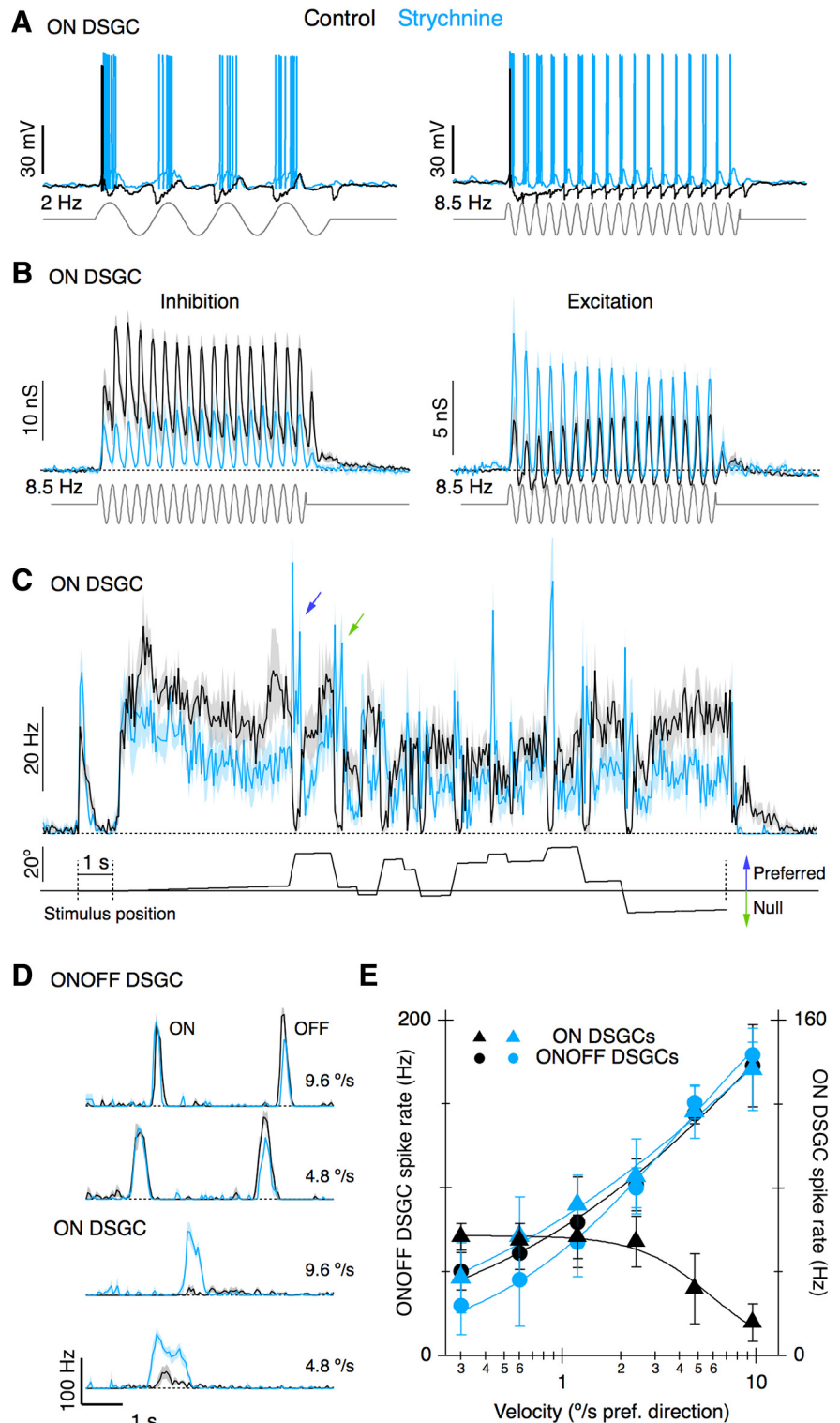
Figure 7. Speed-tuning in ON- and ONOFF-DSGCs is similar after glycinergic block. A , Representative voltage responses during center flicker (diameter, 300 \mu\text{m} ; contrast, 80%) at two frequencies as indicated in control (black; replotted from Fig. 4A) and in the presence of 1 \mu\text{M} strychnine (blue). B , Average synaptic conductances ( n = 4 ) activated by a centered stimulus spot (diameter, 300 \mu\text{m} ; contrast, 80%) modulated at 8.5 Hz, in control (black) and in the presence of 1 \mu\text{M} strychnine (blue). C , PSTHs in response to global drift of a random checkerboard stimulus similar to that shown in Figure 1. Average of six ON-DSGCs in control and during glycinergic block. The arrows highlight preferred and null direction saccades. Spiking increases in both cases. D , PSTHs averaged from four ONOFF-DSGCs and seven ON-DSGCs before (black) and during application of strychnine (blue). Shading shows SEM. Light stimulus was a 300 \mu\text{m} wide bar (same stimulus as Fig. 3B) drifting in the preferred direction at various velocities. Speed of the stimulus indicated next to the traces. E , Peak spike rates shown for the full range of stimulus velocities. Circles show the ON-response of the ONOFF-DSGCs. The scaling of the y-axes is set to normalize the amplitude.
