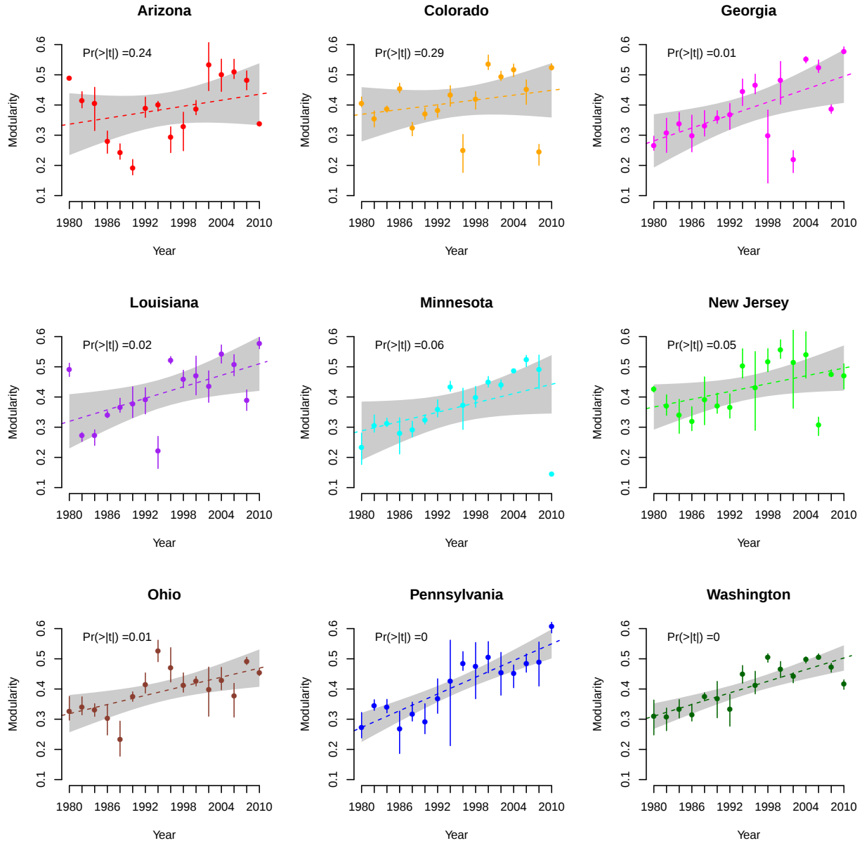
Figure 7.3: Modularity of State Primary Donor Networks
