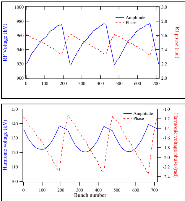
Figure 4: Fundamental (upper) and harmonic (lower) RF voltages and phases.
