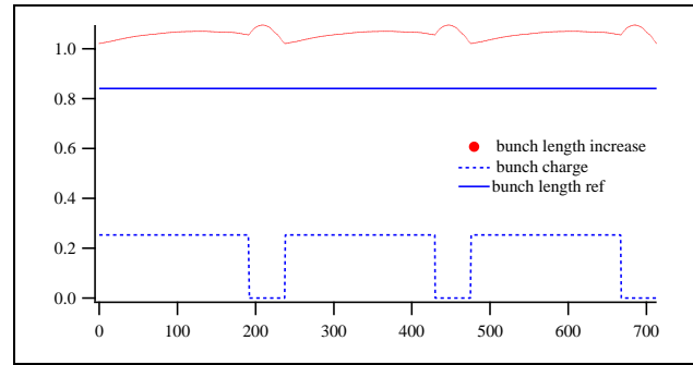
Figure 6: Bunch lengthening.
