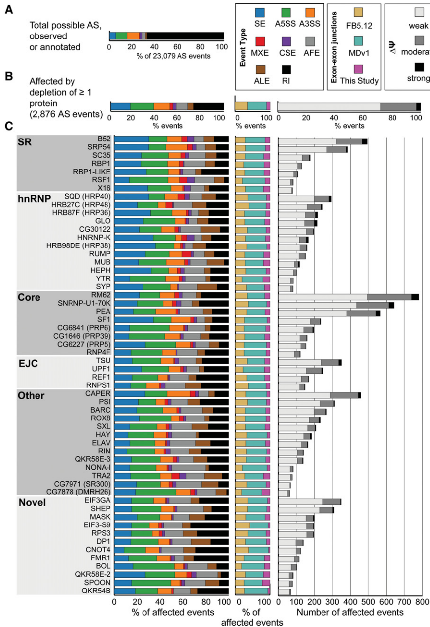
Figure 1. Alternative splicing (AS) events affected by depletion of 56 RNA binding proteins. (A) The proportion of each type of AS event that could potentially be regulated by each protein. (B) The observed proportion of each type of splicing event affected by depletion of at least one protein is shown alongside the type of exon-exon junctions involved in the splicing event. (C) The number, magnitude, type of AS, and type of exon-exon junction affected by each individual knockdown is shown. Each protein is categorized as SR, hnRNP, core splicing factor, exon junction complex (EJC), other known, or novel splicing regulator protein. The legend in the top right indicates the color codes used for the splicing event types. (SE) skipped/cassette exon, (A5SS) alternative 5' splice site, (A3SS) alternative 3' splice site, (MXE) mutually exclusive exons, (CSE) coordinate skipped/cassette exon, (AFE) alternative first exon, (ALE) alternative last exon, (RI) retained intron. In addition, the legend indicates whether the exon-exon junctions were found in FlyBase 5.12, MDv1 (Graveley et al. 2011), or novel to this study, as well as whether the magnitude of splicing changes observed were weak, moderate, or strong.
