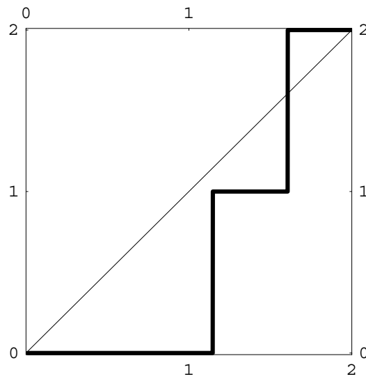
Figure 2: The mapping F for \eta = 0.2 , \phi = .075 , \gamma = 2 , w^B = 3 , \xi^B = 0.6 , and \theta^A = 0.01 .
