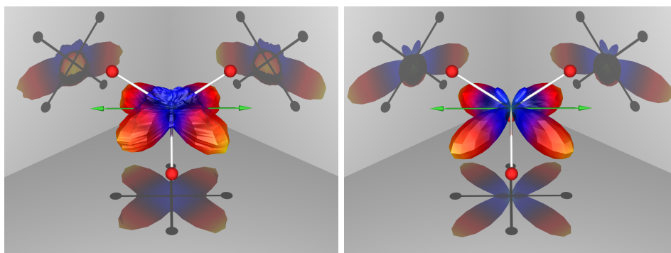
Figure 6: MFPAD for K-shell ionization of \text{CF}_4 with the polarization fixed perpendicular to the \text{C}_2 axis and in the plane of two C-F bonds. Left: the observed photoelectron distribution measured in coincidence with \text{F}^+ + \text{F}^+ following Auger decay. Right: the MFPAD calculated using the complex Kohn variational method. The equilibrium molecular geometry is represented by the ball and stick models and the polarization axis by the double headed arrow.
