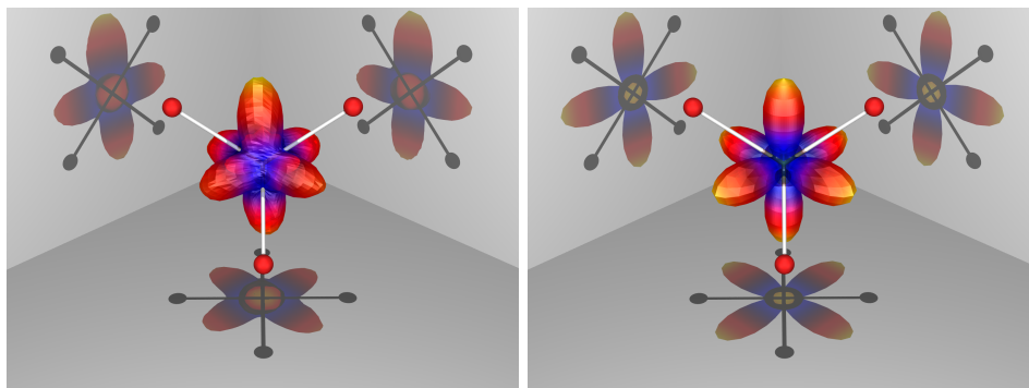
Figure 5: MFPAD for K-shell ionization of \text{CF}_4 . Left: the observed photoelectron distribution measured in coincidence with \text{F}^+ + \text{F}^+ following Auger decay. Right: the MFPAD calculated using the complex Kohn variational method. Data and theory are integrated over all orientations of the polarization vector. The equilibrium molecular geometry is represented by the ball and stick models.
