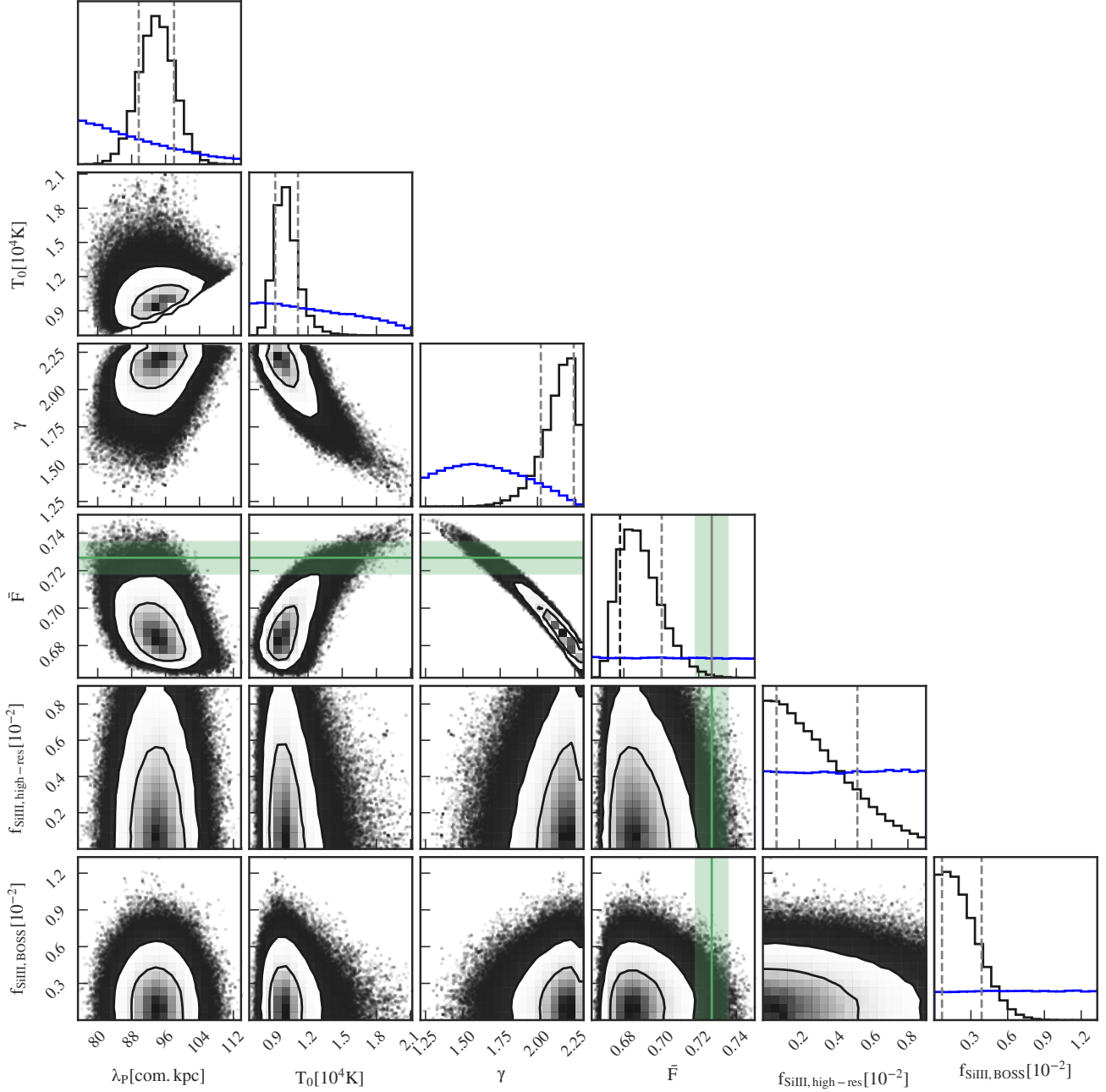
Figure 6. Corner plot showing 1d- and 2d- marginalized posterior distributions for all fitting parameters at z = 2.8 assuming a flat prior on \bar{F} . Blue curves in the 1d-histograms show 1d- marginalized distribution when ignoring the data and fitting the prior only (i.e. the result of the analysis performed for Figure 4). We can see that there are strong constraints on all parameters compared to the prior information. We also notice a strong correlation between permutations of \gamma , T_0 and \bar{F} . Note that the posterior in \bar{F} is significantly below the observed value of the Becker et al. (2013) mean flux measurement (shown as a green line with a band for the 1\text{-}\sigma -region) which is, combined with the strong anticorrelation between \gamma and \bar{F} leading to higher values of \gamma than typically assumed.
