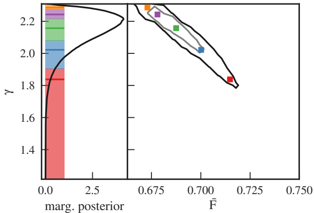
Figure 8. Illustration for our approach in selecting models along the posterior distribution (see main text for details). Left: The marginalized posterior distribution of \gamma values from our chain with the bins which we used to select generate models at the 68% and 95% confidence intervals shown as bars. The median chain value in each bin is shown as a colored line. Right: 68% and 95% contours for \gamma vs. \bar{F} with the selected values of both parameters shown as squares.
