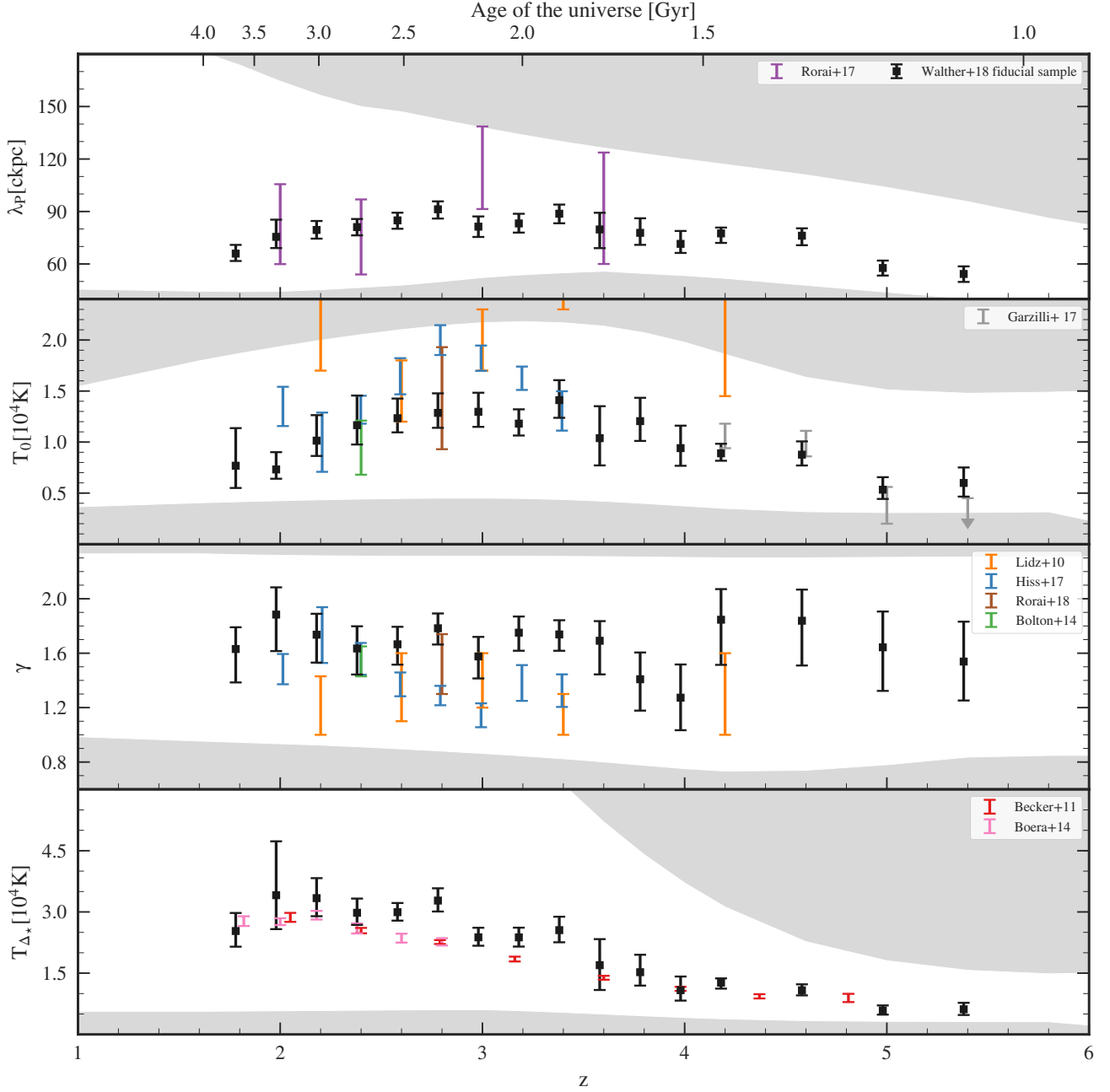
Figure 15. The fiducial data from Figure 13 (black points) assuming the strong Gaussian prior on \bar{F} . In addition to the previous plots we show the thermal parameters as well as T(\Delta_*) at the optimal overdensities \Delta_* for curvature measurements as given by Becker et al. (2011). We compare to measurements of thermal evolution in the IGM based on different statistics: curvature (red, pink), line fitting (green, blue, brown), wavelets (orange), phase angles (purple) and power spectrum (gray). We can see overall good agreement with previous datasets (except for wavelets) albeit significantly higher T(\Delta_*) than in the curvature measurements is obtained at some redshifts. All measurement errors shown are 1\sigma or 68% intervals, for measurements that only quote 2\sigma errorbars we divided those by a factor of two.
