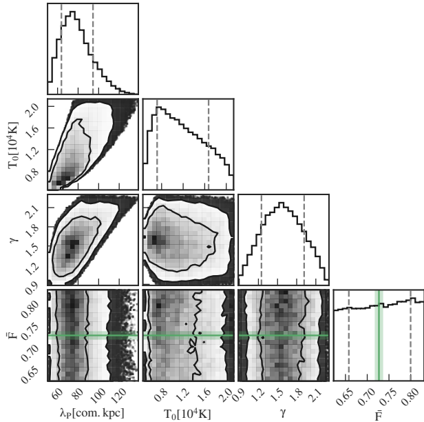
Figure 4. Corner plot showing the Prior PDF for thermal parameters and \bar{F} given our model grid and excluding parameter values outside its convex hull. This was obtained by sampling our prior with an MCMC assuming a flat likelihood. Note that the degeneracies in our model grid lead to non-flat marginalized distributions. The diagonal shows the 1d-PDF (marginalized over all other parameters) for each parameter with dashed vertical lines at the 16% and 84% quantiles. The scatter plots below show the 2d-PDFs for each combination of 2 parameters (also marginalized over all others) with contours showing the region containing the 68% and 95% highest densities. Note that due to the restrictions of our grid there is a strong correlation especially between T_0 and \lambda_P . The additional preference towards low T_0 or \lambda_P is due to our choice of flat priors in the log of these parameters. The green band shows the 1\sigma interval in \bar{F} we use for the Gaussian prior.
