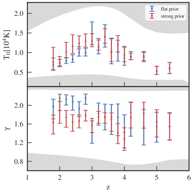
Figure 14. Comparison of our results on the thermal state dependent on redshift between both priors (different colors). We can see that the flat prior leads to far higher values of \gamma that due to correlations between parameters lead to lower values of T_0 ).
