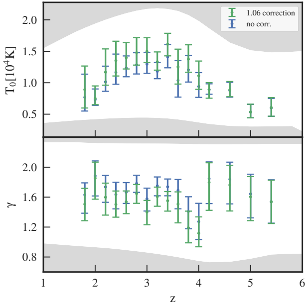
Figure 18. Comparison of our results on the thermal state with fits obtained if we apply a flat “correction factor” of 0.94 (mimicking the joint effect of box size and cosmic variance seen in Figure 17 ) to the model power (different colors). We can see that without the “correction” higher values of \gamma as well as lower values of T_0 (due to correlations between parameters) are obtained.
