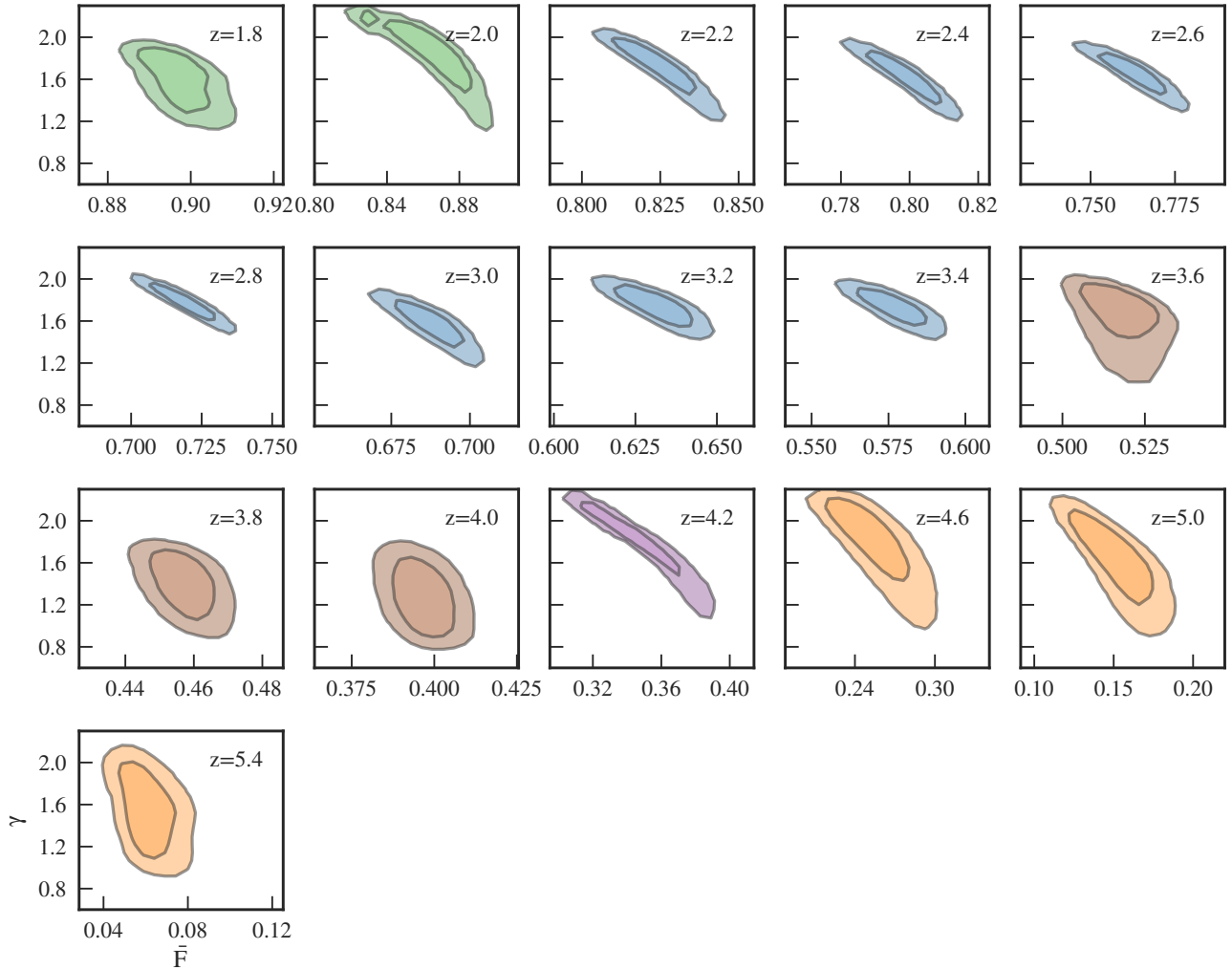
Figure 12. The same as Figure 11 but with \bar{F} vs. \gamma contours. This shows that independent of redshift \gamma and \bar{F} are strongly anticorrelated.
