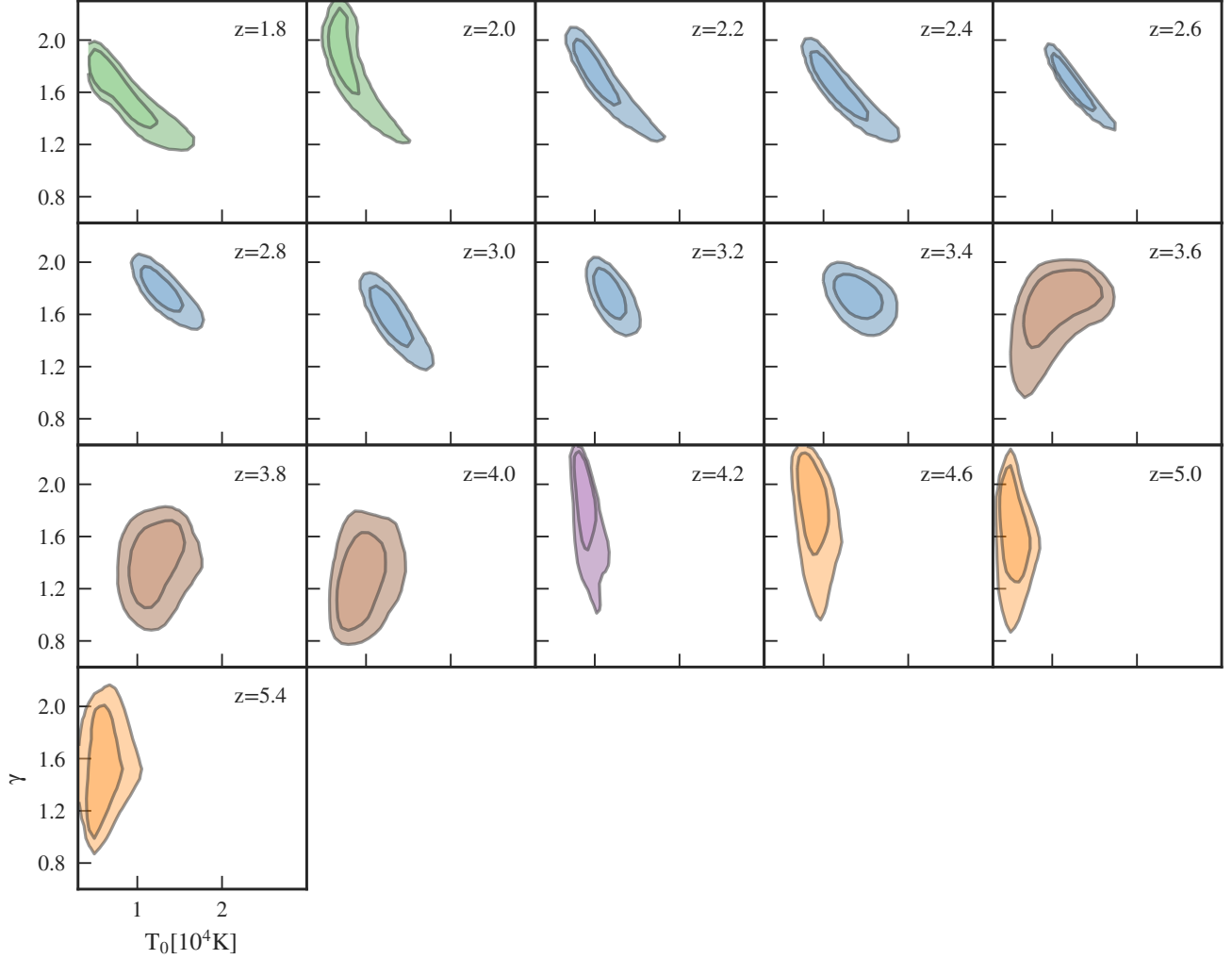
Figure 11. Evolution of the T_0 vs \gamma contours with redshift assuming the strong prior on \bar{F} for different combinations of datasets (different colors matched to Figure 7, filled contours showing our fiducial dataset while open contours show analyses ignoring the XQ-100 data as in the circles of Figure 7). When high resolution data is used we can see that strong constraints perpendicular to a degeneracy direction can be obtained. We can also see that this degeneracy direction rotates as the Ly \alpha forest probes higher and higher densities.
