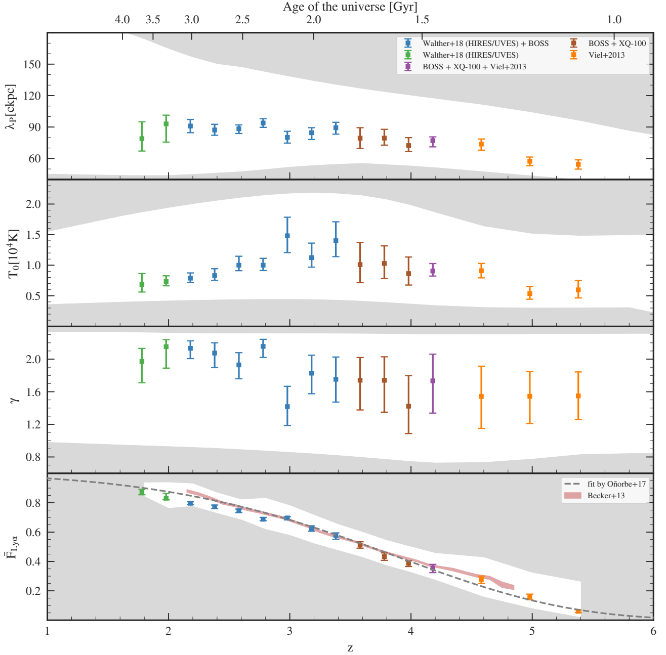
Figure 7. Points with error bars show the median and the region between 16% and 84% quantiles of the 3 thermal parameters as well as the mean transmission of the IGM (marginalized over all model parameters of the fit) at different redshifts using our fiducial dataset (squares) at each redshift. In the \bar{F} panel we also show the evolution obtained by Becker et al. (2013) (red band showing 1\sigma uncertainties) based on relative changes in SDSS quasar transmissions as well as the Oñorbe et al. (2017a) (dashed line) fit to these data and further datasets. Note the large discrepancies between our measurements and those results when assuming an uninformative prior on the mean flux. The white range shows the space populated by our models, i.e. we cannot expect to measure values inside the gray shade using our current emulator.
