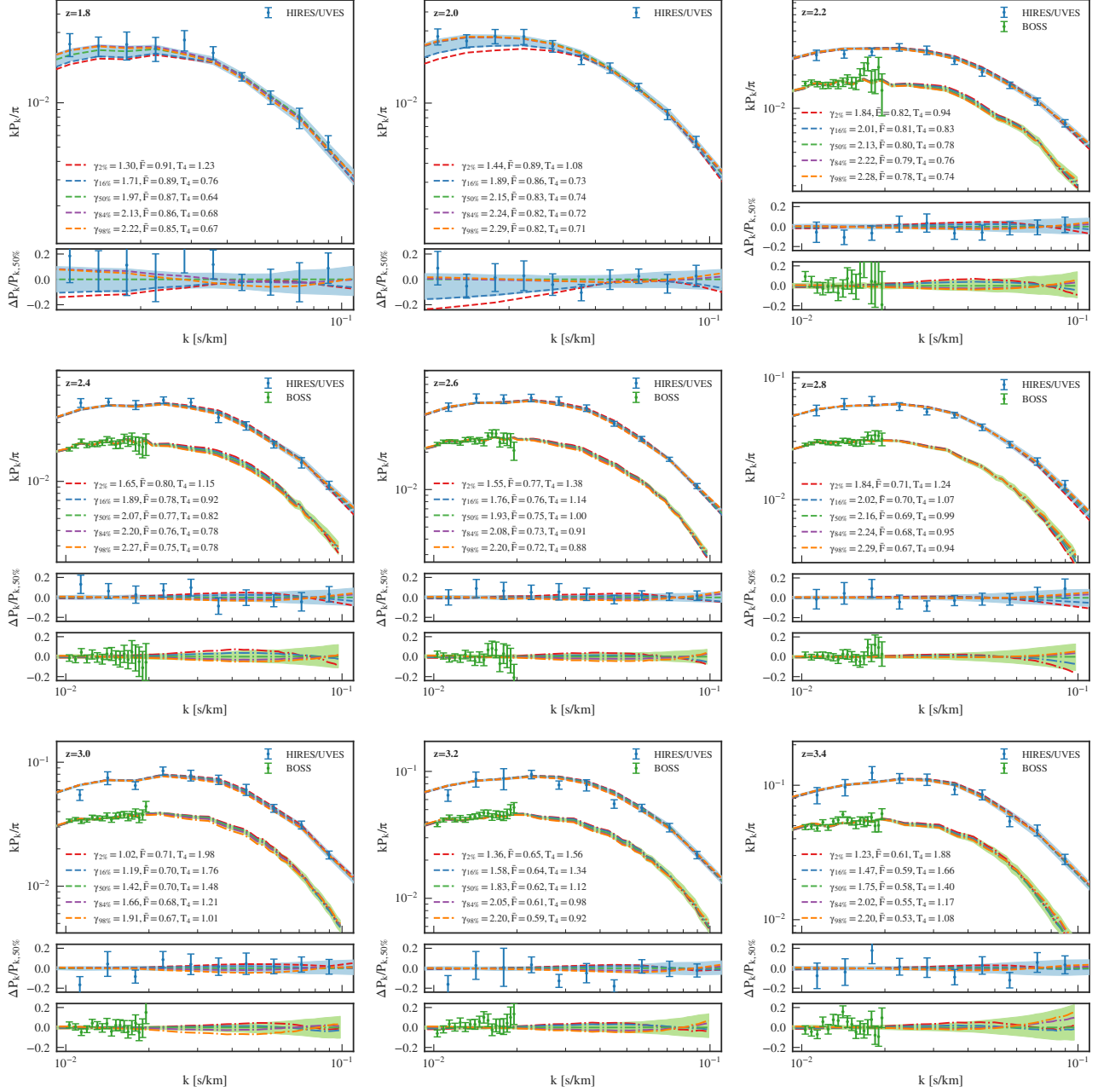
Figure 10. Same as Figure 9, but also for all redshifts z \leq 3.4 . We can see that while most redshift bins show the strongest scatter in the power at k \sim 0.06 \text{ s km}^{-1} when moving along the degeneracy direction. However, for z = 1.8, 2.0 the behaviour seems to be significantly different most likely due to the lacking precision on small k due to the lack of the BOSS measurement at these redshifts.
