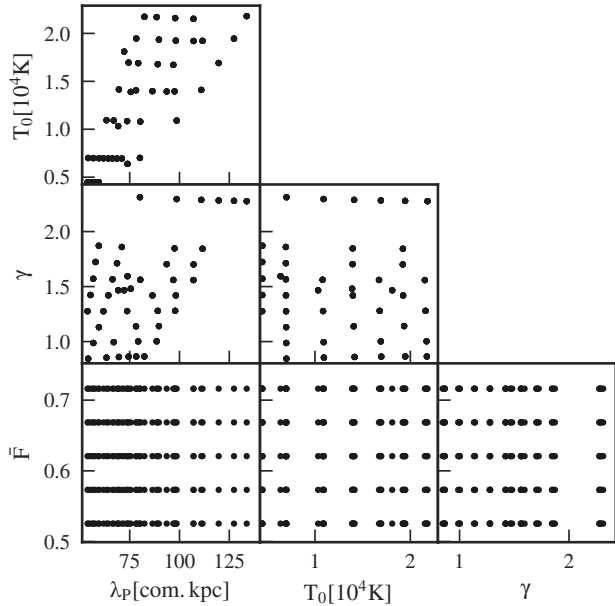
Figure 2. The subset of thermal models we used at z = 3.2 . Each point in the T_0, \gamma, \lambda_P space corresponds to a different Hydrodynamical simulation. Note the correlations between T_0 ( \gamma ) and \lambda_P in the grid. For each simulation we rescaled the optical depths to obtain outputs with different mean transmitted fluxes \bar{F} .
