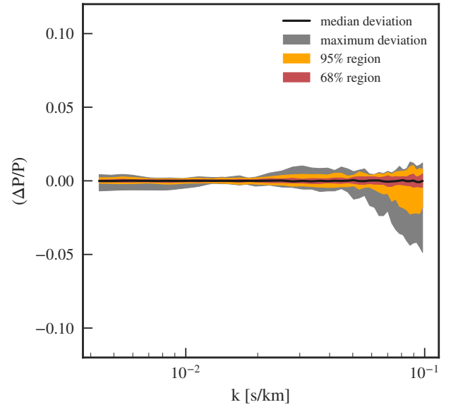
Figure 3. Cross validation results for our emulation procedure at z = 2.8 . Colored bands are showing the relative difference between emulated and true power for different cuts of the full cross validation set. The median is shown as a black curve. Other redshifts give similar results especially for the 68% region. See main text for more details.
