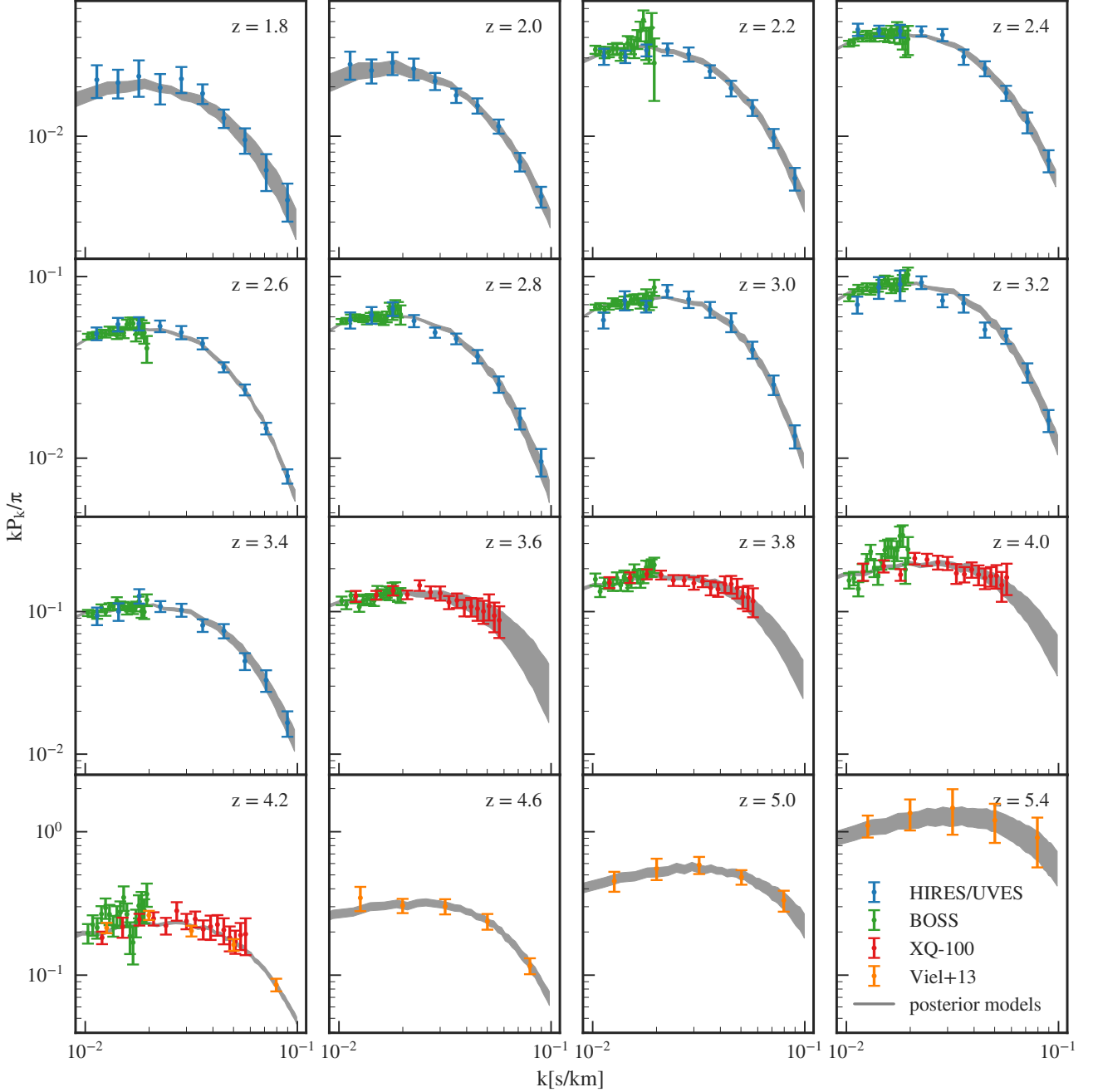
Figure 5. Redshift evolution of the power spectrum with colors showing different datasets. Data by Iršič et al. (2017a) were corrected to the median of the marginalized posterior resolution, Walther et al. (2018) points have been corrected for the masking window function. All data have been corrected for Si III correlations. Bands show 68% confidence regions for our emulator with parameters randomly drawn from the posterior distribution.
