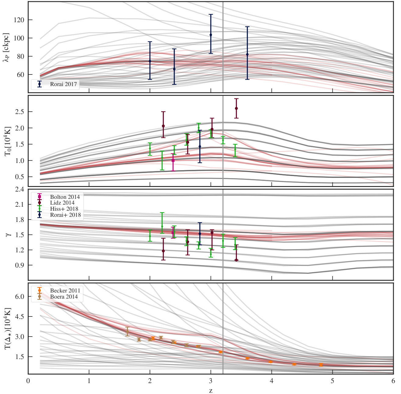
Figure 1. Redshift evolution of different thermal evolution models (lines). Most of the different curves (gray) were obtained by changing the overall heating rates from (Haardt & Madau 2012) by a factor (changing T_0 at all redshifts) as well as the exponent in their density dependence (changing \gamma at all redshifts) according to eqn. (2). As the pressure smoothing scale \lambda_P is dependent on the full thermal evolution of the IGM it changes accordingly in these cases. Additional models of thermal evolution (red) with different H I and He II reionization redshifts and heat inputs partially break those degeneracies. Also shown is the Temperature T(\Delta_*) (based on the values of \Delta_* by Becker et al. 2011) at the overdensity where constraints from curvature measurements are independent of \gamma . We compare to the measurements by Lidz et al. (2010), Becker et al. (2011), Bolton et al. (2014), Boera et al. (2014), Rorai et al. (2017b), Hiss et al. (2018) and Rorai et al. (2018) in the parameters constrained by the respective analysis. The Lidz et al. (2010), Bolton et al. (2014) and Rorai et al. (2018) data have been offset by 0.02 along the redshift axis for clarity.
