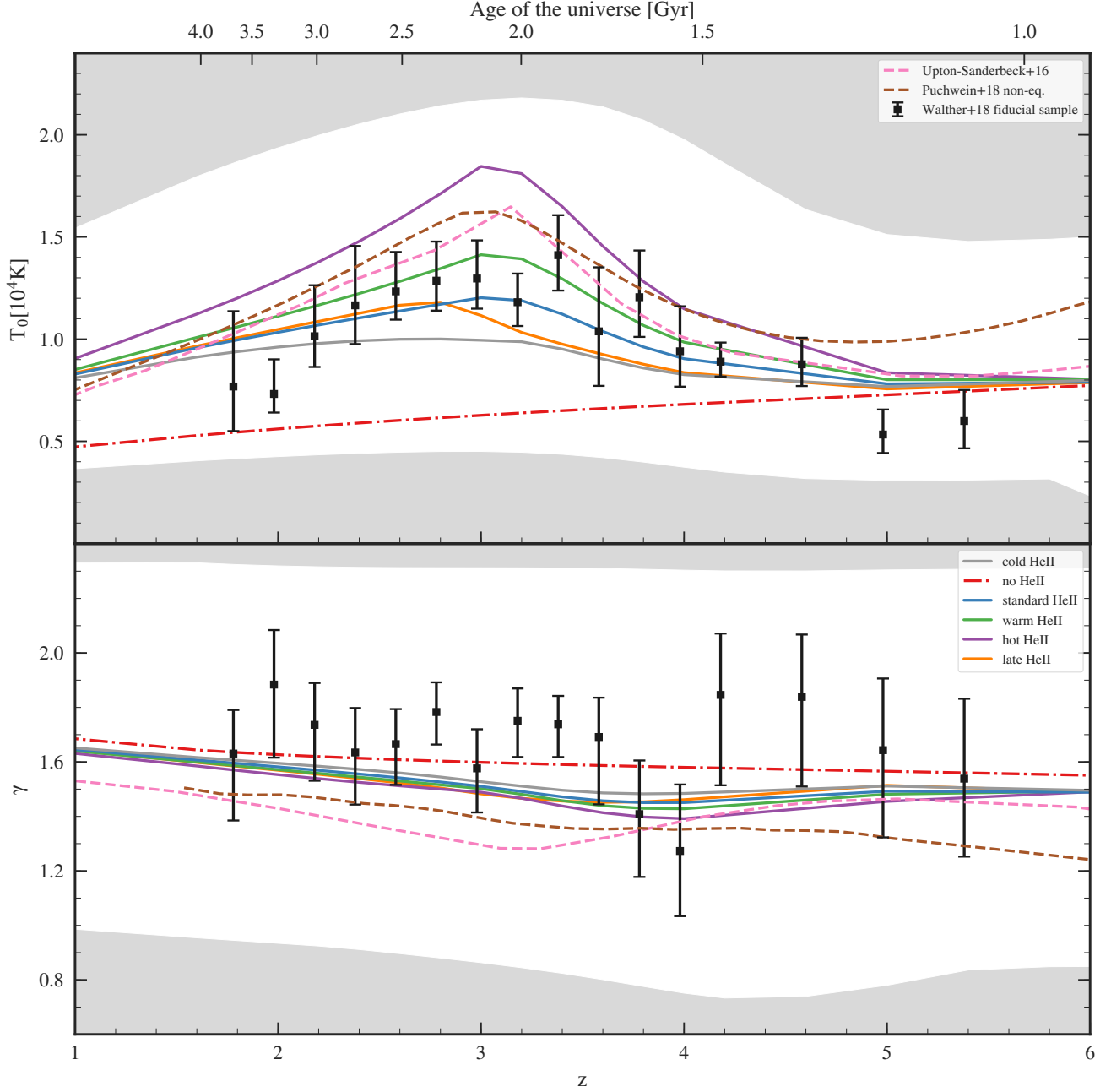
Figure 16. The fiducial data assuming the strong Gaussian prior from Figure 13 (black points) compared to thermal evolution models assuming different redshifts of He II reionization and heat inputs during this process (solid curves) and without any He II reionization (dot-dashed red curve). The model parameters are given in Table 2. We also show comparisons to the Upton Sanderbeck et al. (2016) (dashed pink) thermal evolution model and a run using the Puchwein et al. (2018) non-eq. heating rates in a Nyx simulation (dashed brown). We can clearly see that the data shows a hotter IGM than created in the model without He II reionization. Instead, the overall evolution of thermal parameters seems to agree well with the standard to warm He II reionization scenarios in both T_0 and \gamma . Finally, the temperatures found at the 2 highest redshift bins are colder than any model.
