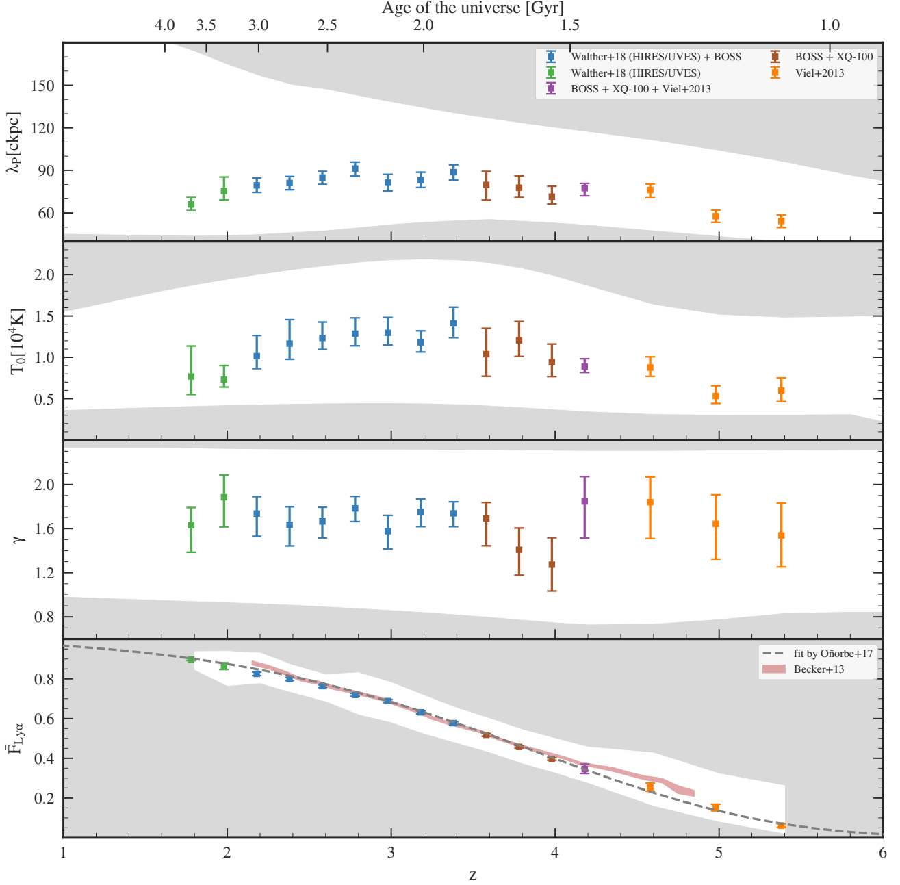
Figure 13. The fiducial measurements from Figure 7, but assuming a Gaussian prior on the mean transmission complying with the fit of (Oñorbe et al. 2017b) measurement within errorbars given by observations (Becker et al. 2013; Faucher-Giguère et al. 2008a; Kirkman et al. 2005). We can see that now the obtained \gamma values at low redshifts are far lower (and compatible with the expected value of 1.6 long after reionization) due to the additional mean transmission constraint. The high values of \gamma at high redshifts obtained here, are likely due to the discrepancy of the mean of our chosen prior (dashed curve) with the Becker et al. (2013) (red band) analysis for the mean transmission. Due to the far lower overdensities probed at high-redshifts compared to low redshifts these high values of \gamma do not change results on T_0 strongly as degeneracies are largely broken (see also the evolution of the T_0 - \gamma and \gamma - \bar{F} contours which can be found in Figure 11 and Figure 12 ).
