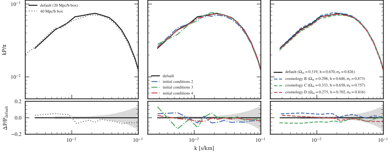
Figure 17. Left: One model from our thermal grid at z = 2.8 (solid black, the redshift is taken as an example, other redshifts are similar) compared to the same model run with a two times larger box and the same spatial resolution (dotted gray). The bottom panel shows relative differences and the size of the 68% confidence region of jointly fitting BOSS + high-resolution data as a grey band. Center: A comparison between different initial conditions (dot-dashed) that were otherwise run with the same setup. Right: A comparison of models based on other cosmologies (B,C are compatible with the Planck Collaboration et al. 2016a parameters and chosen to maximally change the matter power spectrum w.r.t. the default model, see Oñorbe et al. 2017a for details; D is the cosmology from Lukić et al. 2015 ). We can see that all three effects change the power on the 5% level.
