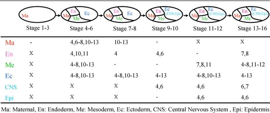
Figure 2 A spatiotemporal sequence of network motifs of the D. melanogaster developmental gene network. 'X' denotes the region where we could not apply our network motif identification due to the absence of active sub-network and '-' denotes the region where we did not identify any network motif. '(CNS, Epi)' in the ellipse indicates that the two regions CNS and Epi are differentiated from Ec and located inside Ec.
