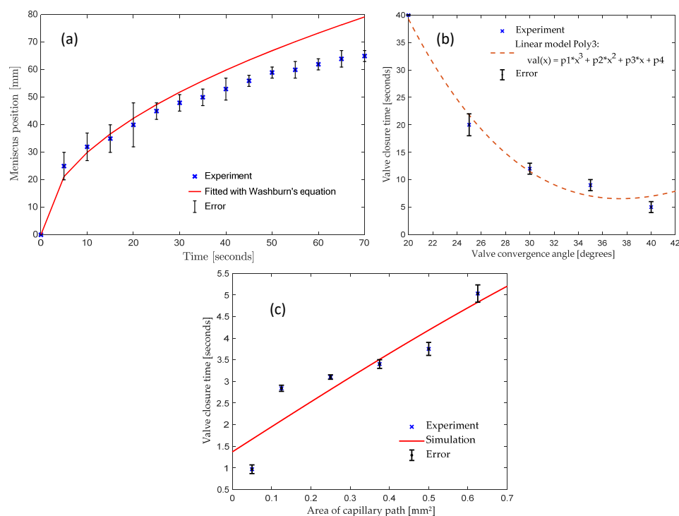
Figure 8. (a) Plot of the time of vs. advancement of the molten ferrowax meniscus in the fluidic channel under capillary action. The experimental values are indicated by blue cross marks (where the error bars represent one standard deviation). The red line indicates the trend corresponding to Washburn's Equation (Equation (9), with W = 9.47 ). The simulation predictions of the molten wax location (Washburn's Equation) are within 18.75% of the error margin with respect to experimental results. (b) Plot depicting the relationship between the valve convergence angle (see Figure 3b for definition) and the time it takes for the molten wax to reach the fluidic channel. The error bars represent one standard deviation. Dotted line is a fitted curve to the blue crosses. (c) Relationship between the valving channel cross-section and the response time. The red line shows the simulated curve and blue crosses represent experimental measurements done using the Hamilton syringe setup where we use a Hamilton syringe to input the wax.
