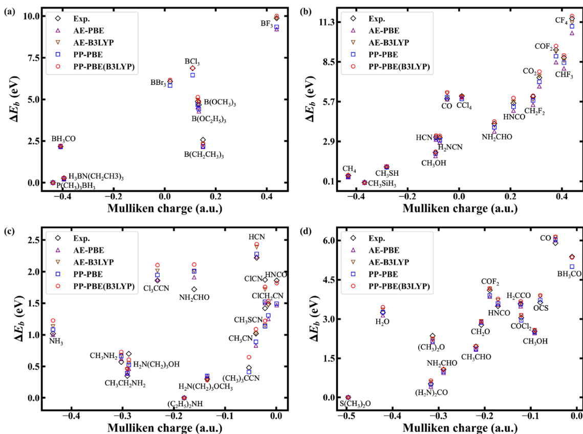
Figure 4. Binding energy shifts versus the Mulliken charges of molecules for (a) B, (b) C, (c) N, and (d) O core excitations.
