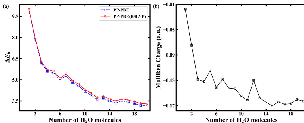
Figure 5. (a) The binding energy shifts of the O-1s core level for protonated water with respect to that of an isolated water molecule. (b) The Mulliken charge on the O atom in protonated water.
