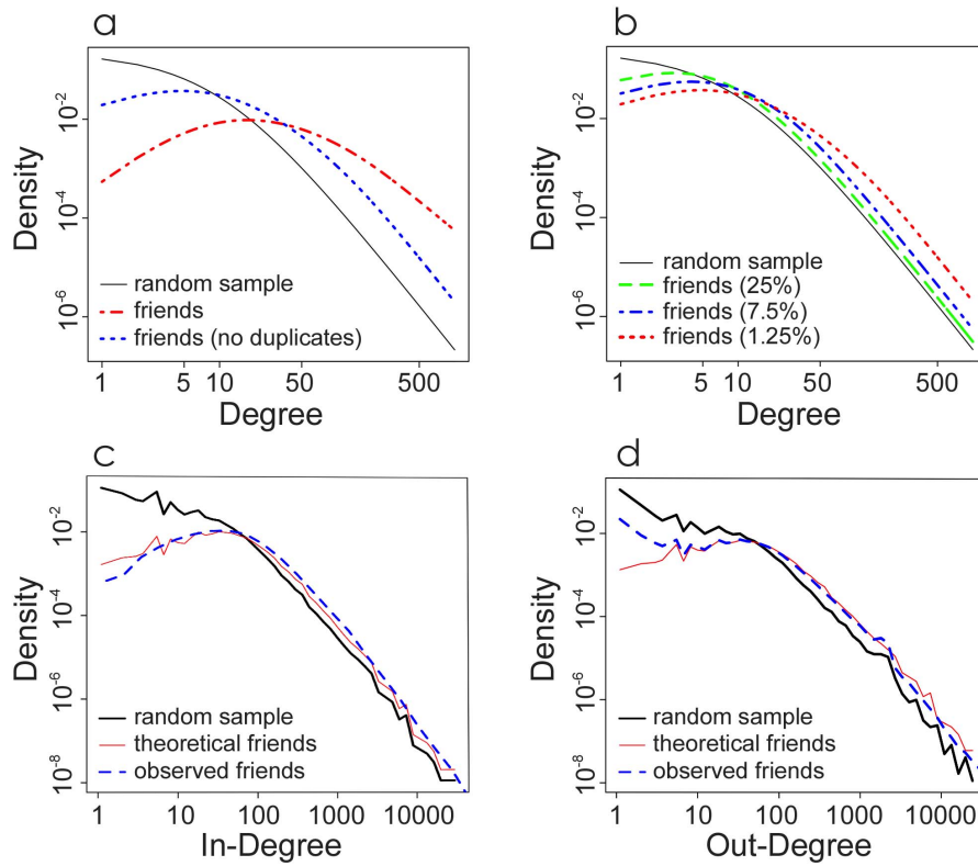
Figure 1. Twitter exhibits the “friendship paradox”. a) Expected degree distributions for a 1.25% random sample of the Twitter network (black line), friends of this randomly chosen group (red line), and the same friends group with duplicates removed (blue line); b) Larger samples of friends show a smaller difference in degree distribution from the overall network (black=overall network, green=25% sample, blue=7.5% sample, red=1.25%); c) and d) Respectively, In-degree (follower) and out-degree (followee) distribution of a random sample of 500,000 users, 1.25% of Twitters users (the “control” group, black line) and the theoretical (red line) and observed (blue line) in-degree and out-degree distributions of their friends (the “sensor” group) with duplicates from the friends group removed. doi:10.1371/journal.pone.0092413.g001
