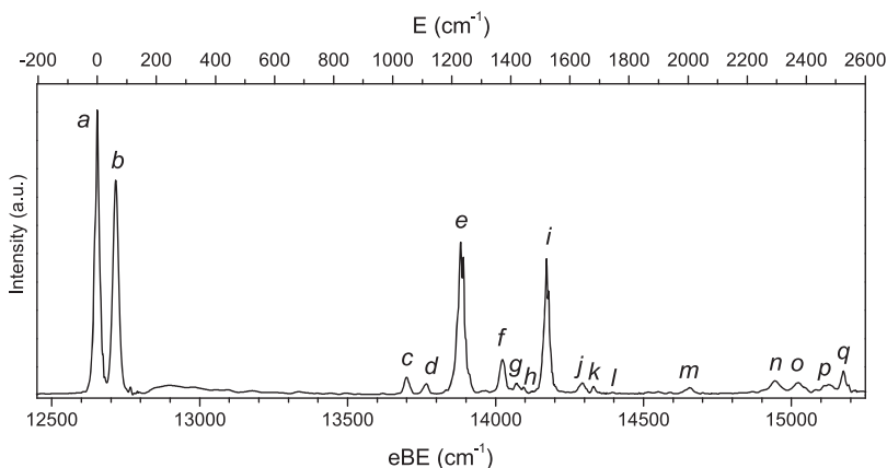
FIG. 1. Cryo-SEVI spectrum of CH 3 O. The energy scale is shown in cm -1 for both electron binding energy (eBE) and energy relative to the vibrational origin (E).
