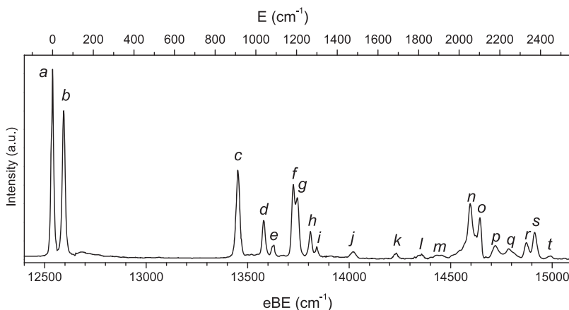
FIG. 2. Cryo-SEVI spectrum of \text{CD}_3\text{O} . The energy scale is shown in \text{cm}^{-1} for both electron binding energy (eBE) and energy relative to the vibrational origin (E).
