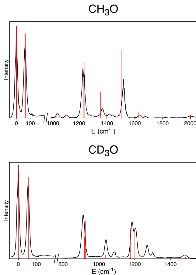
FIG. 4. Cryo-SEVI spectra of \text{CH}_3\text{O} and \text{CD}_3\text{O} (black) and simulated spectra using the KDC model Hamiltonian (red sticks). The maximum quantum number for basis functions in each mode is (5, 6, 6, 5, 5, 6, 6, 9, 9) for \text{CH}_3\text{O} and (4, 7, 7, 4, 4, 7, 7, 8, 8) for \text{CD}_3\text{O} . Spectra are plotted in \text{cm}^{-1} relative to the position of the vibrational origin at 12\,654\text{ cm}^{-1} for \text{CH}_3\text{O} and 12\,543\text{ cm}^{-1} for \text{CD}_3\text{O} .
