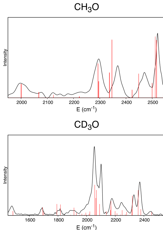
FIG. 5. Cryo-SEVI spectra of \text{CH}_3\text{O} and \text{CD}_3\text{O} (black) showing the higher-lying vibronic structure and simulated spectra using the KDC model Hamiltonian (red sticks). The maximum quantum number for basis functions in each mode is (5, 6, 6, 5, 5, 6, 6, 9, 9) for \text{CH}_3\text{O} and (4, 7, 7, 4, 4, 7, 7, 8, 8) for \text{CD}_3\text{O} . Spectra are plotted in \text{cm}^{-1} relative to the position of the vibrational origin at 12\,654\text{ cm}^{-1} for \text{CH}_3\text{O} and 12\,543\text{ cm}^{-1} for \text{CD}_3\text{O} .
