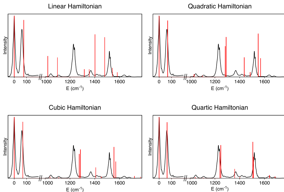
FIG. 3. Cryo-SEVI spectra of \text{CH}_3\text{O} (black) and simulated spectra using the KDC model Hamiltonian (red sticks). The maximum quantum number for basis functions in each mode is (3, 6, 6, 3, 3, 6, 6, 6, 6). Spectra are plotted in \text{cm}^{-1} relative to the position of the vibrational origin at 12\,654\text{ cm}^{-1} .
