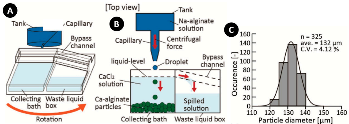
Figure 12. (A,B) Conceptual illustration of oil-free production of monodisperse Ca-alginate particles with a by-pass channel and waste chamber for transferring spilled solution in order to keep the CaCl 2 solution level constant; (C) Diameter distribution of Ca-alginate particles. Reprinted with permission from [121].
