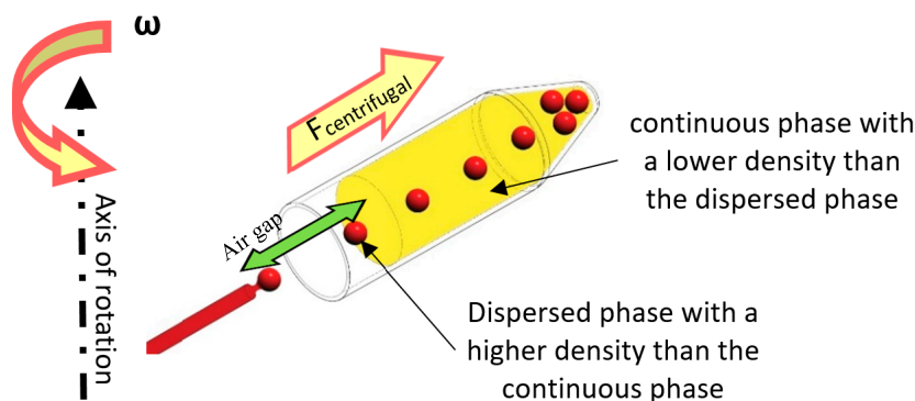
Figure 6. Schematic view of the dispenser nozzle method for droplet and particle generation. Droplets are produced at the tip of the nozzle and enter a tube containing a continuous phase.
