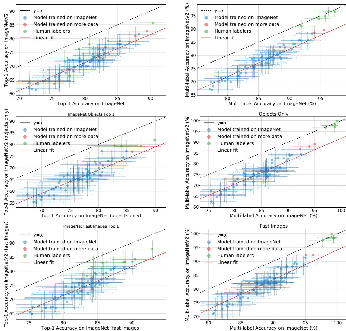
Figure 3.6: (left) \tau_{\text{top-1}} accuracies and (b) multi-label accuracies for both convolutional neural networks and five human labelers on the ImageNet validation set versus their accuracies on the ImageNetV2 test set. The confidence intervals are 95% Clopper-Pearson confidence intervals.
